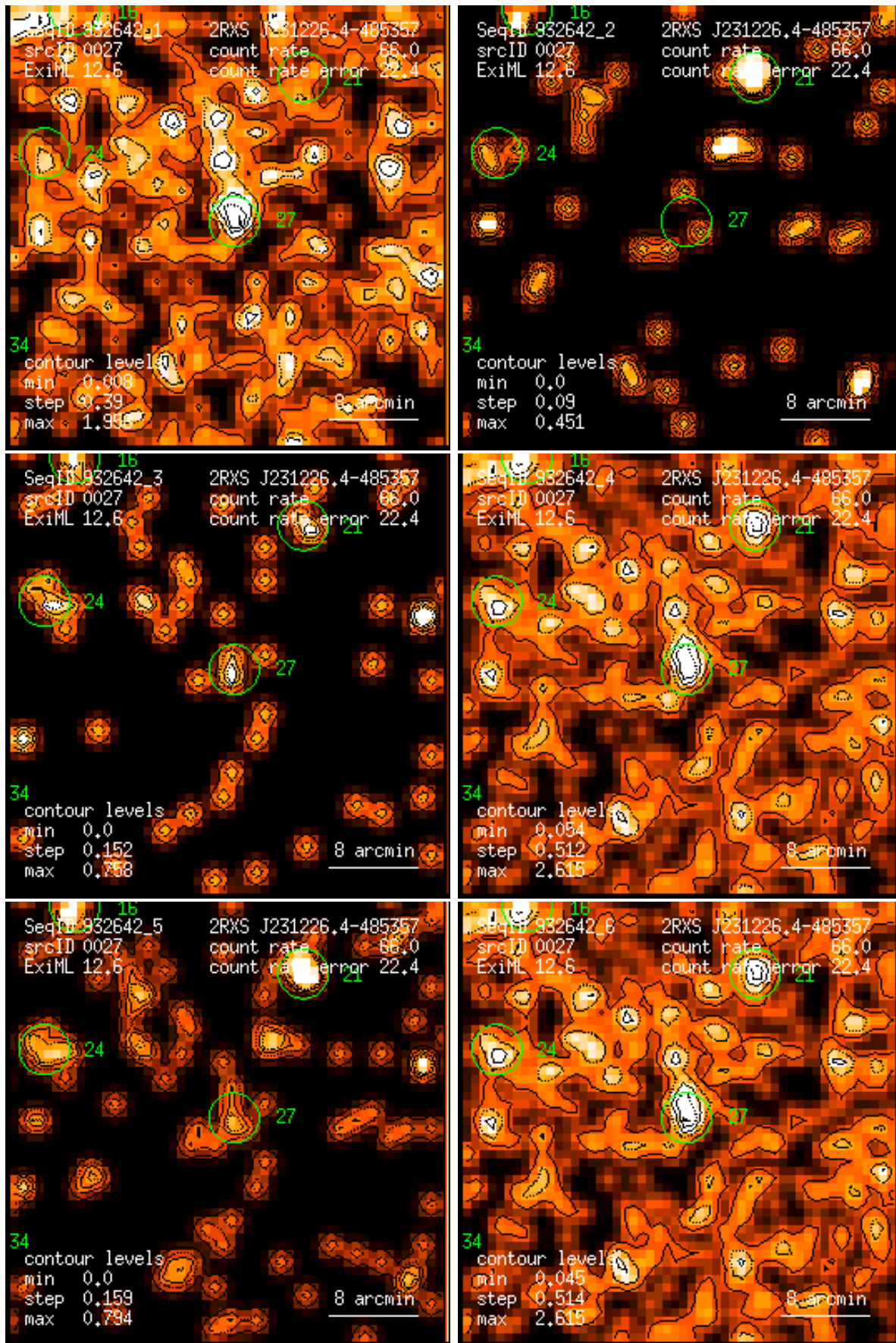
Figure 27: RASS 932642: detection 0027: band rate images, Gaussian filter: (1) PSPC channels 11 – 41, (2) 52 – 90, (3) 91 – 201, (4) 11 – 235, (5) 52 – 201, (6) 11 – 201. Broad band rates in counts/ks. Band rate contour levels in counts/ks/arcmin 2 .
