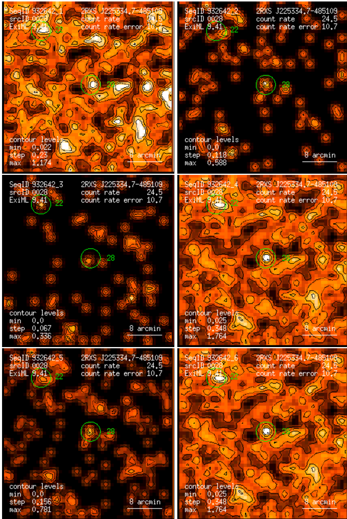
Figure 28: RASS 932642: detection 0028: band rate images, Gaussian filter: (1) PSPC channels 11 – 41, (2) 52 – 90, (3) 91 – 201, (4) 11 – 235, (5) 52 – 201, (6) 11 – 201. Broad band rates in counts/ks. Band rate contour levels in counts/ks/arcmin 2 .
