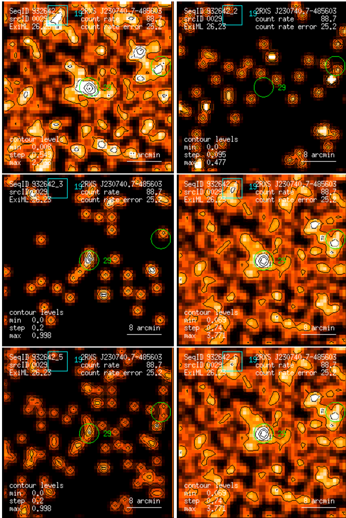
Figure 29: RASS 932642: detection 0029: band rate images, Gaussian filter: (1) PSPC channels 11 – 41, (2) 52 – 90, (3) 91 – 201, (4) 11 – 235, (5) 52 – 201, (6) 11 – 201. Broad band rates in counts/ks. Band rate contour levels in counts/ks/arcmin 2 .
