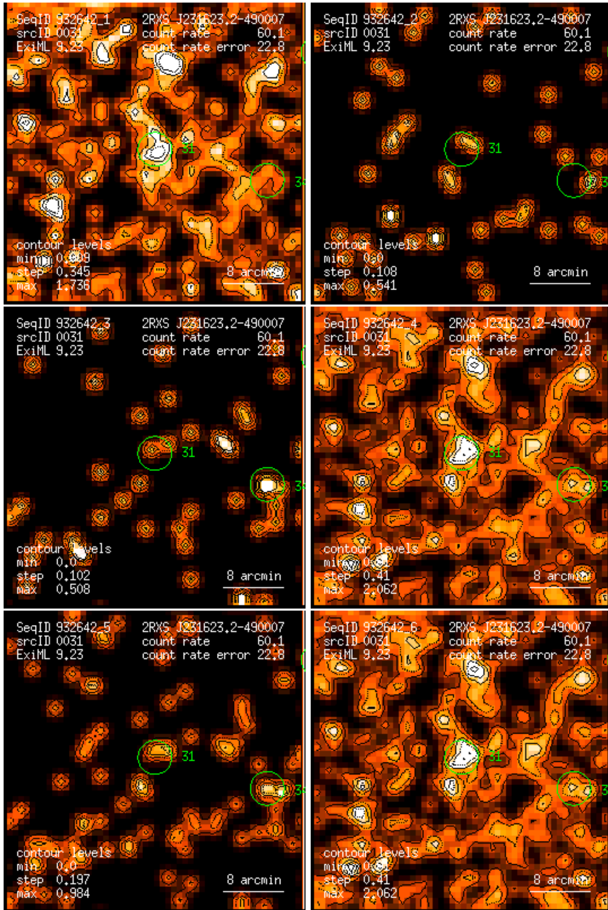
Figure 31: RASS 932642: detection 0031: band rate images, Gaussian filter: (1) PSPC channels 11 – 41, (2) 52 – 90, (3) 91 – 201, (4) 11 – 235, (5) 52 – 201, (6) 11 – 201. Broad band rates in counts/ks. Band rate contour levels in counts/ks/arcmin 2 .
