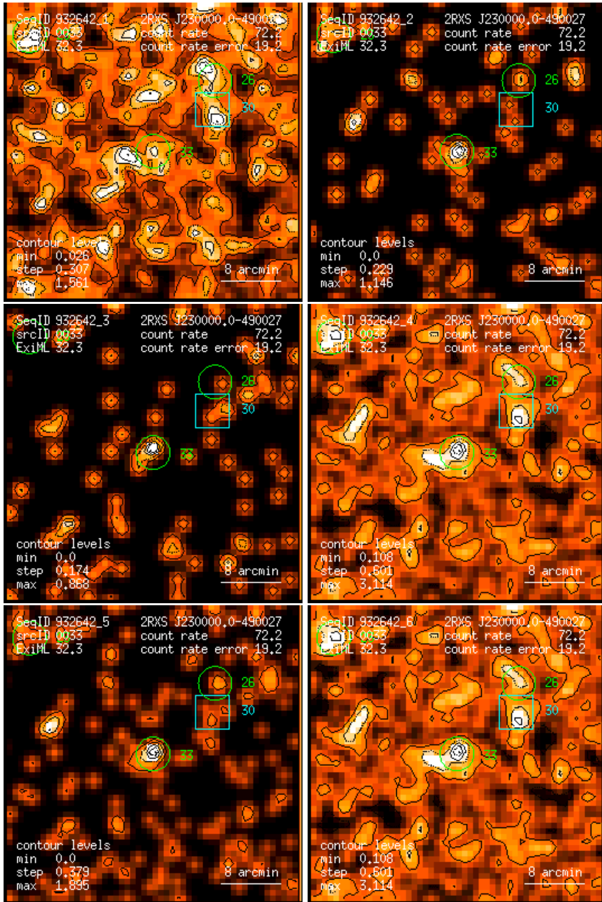
Figure 33: RASS 932642: detection 0033: band rate images, Gaussian filter: (1) PSPC channels 11 – 41, (2) 52 – 90, (3) 91 – 201, (4) 11 – 235, (5) 52 – 201, (6) 11 – 201. Broad band rates in counts/ks. Band rate contour levels in counts/ks/arcmin 2 .
