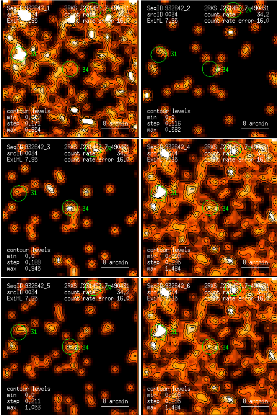
Figure 34: RASS 932642: detection 0034: band rate images, Gaussian filter: (1) PSPC channels 11 – 41, (2) 52 – 90, (3) 91 – 201, (4) 11 – 235, (5) 52 – 201, (6) 11 – 201. Broad band rates in counts/ks. Band rate contour levels in counts/ks/arcmin 2 .
