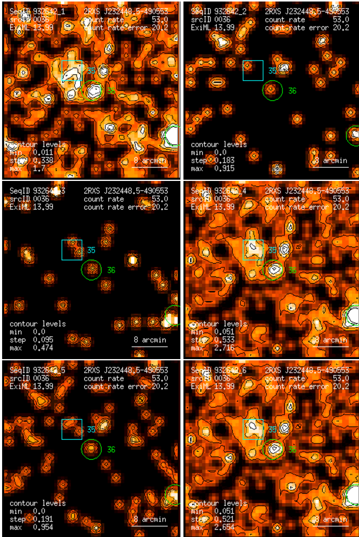
Figure 36: RASS 932642: detection 0036: band rate images, Gaussian filter: (1) PSPC channels 11 – 41, (2) 52 – 90, (3) 91 – 201, (4) 11 – 235, (5) 52 – 201, (6) 11 – 201. Broad band rates in counts/ks. Band rate contour levels in counts/ks/arcmin 2 .
