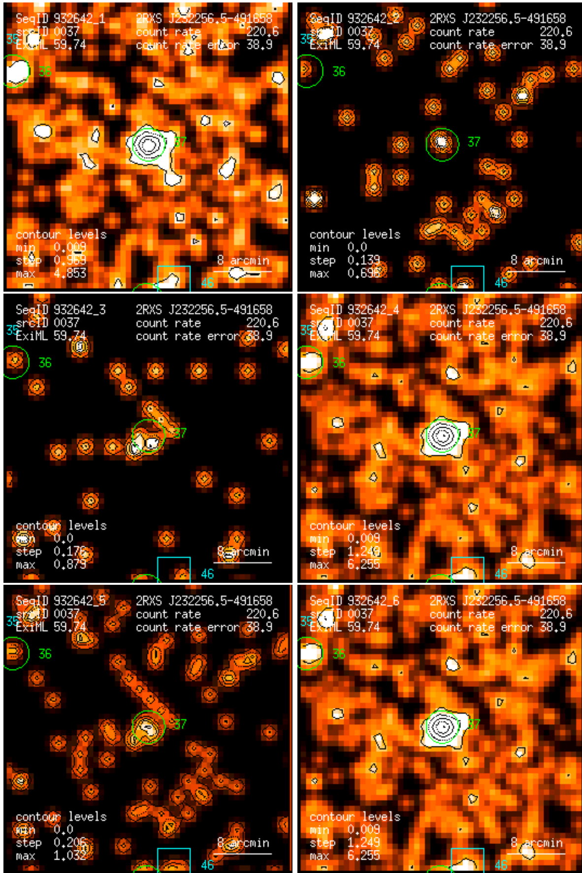
Figure 37: RASS 932642: detection 0037: band rate images, Gaussian filter: (1) PSPC channels 11 – 41, (2) 52 – 90, (3) 91 – 201, (4) 11 – 235, (5) 52 – 201, (6) 11 – 201. Broad band rates in counts/ks. Band rate contour levels in counts/ks/arcmin 2 .
