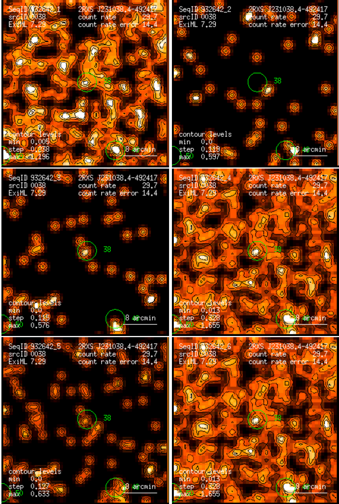
Figure 38: RASS 932642: detection 0038: band rate images, Gaussian filter: (1) PSPC channels 11 – 41, (2) 52 – 90, (3) 91 – 201, (4) 11 – 235, (5) 52 – 201, (6) 11 – 201. Broad band rates in counts/ks. Band rate contour levels in counts/ks/arcmin 2 .
