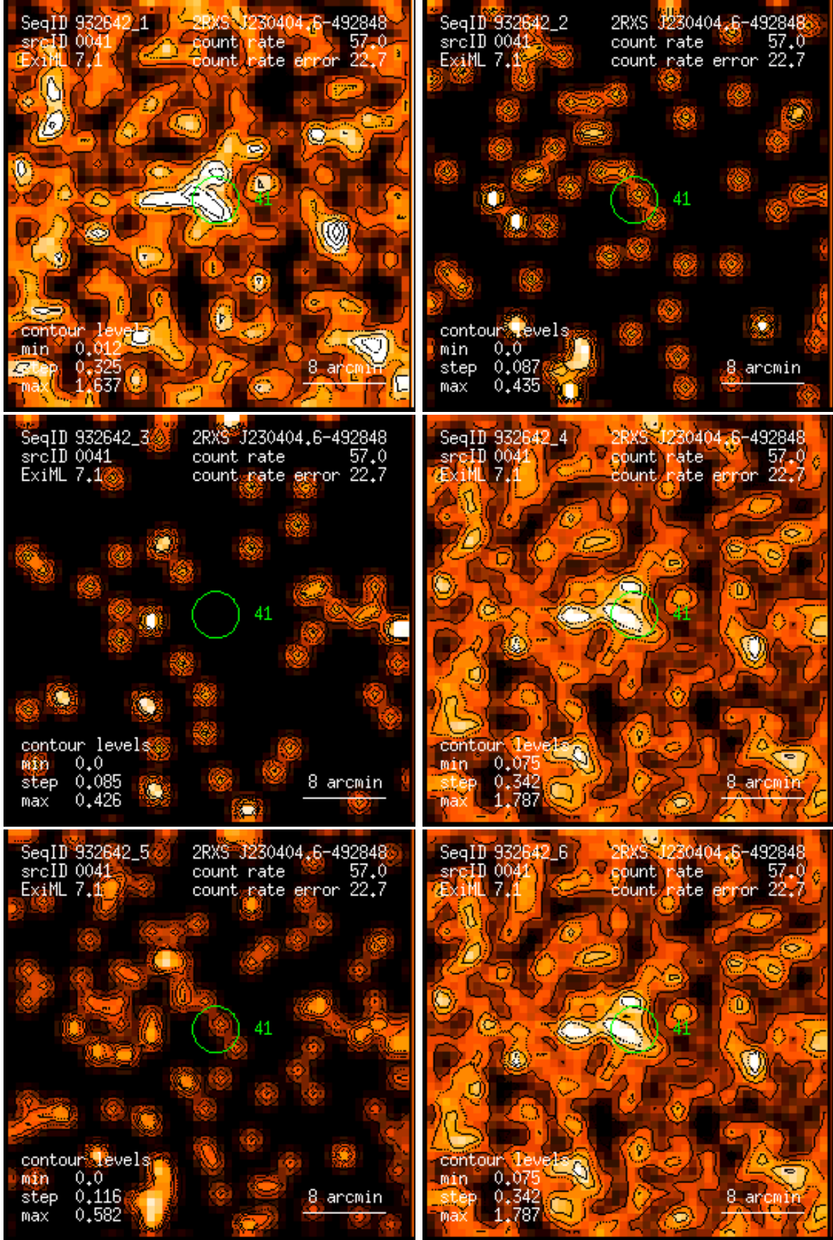
Figure 41: RASS 932642: detection 0041: band rate images, Gaussian filter: (1) PSPC channels 11 – 41, (2) 52 – 90, (3) 91 – 201, (4) 11 – 235, (5) 52 – 201, (6) 11 – 201. Broad band rates in counts/ks. Band rate contour levels in counts/ks/arcmin 2 .
