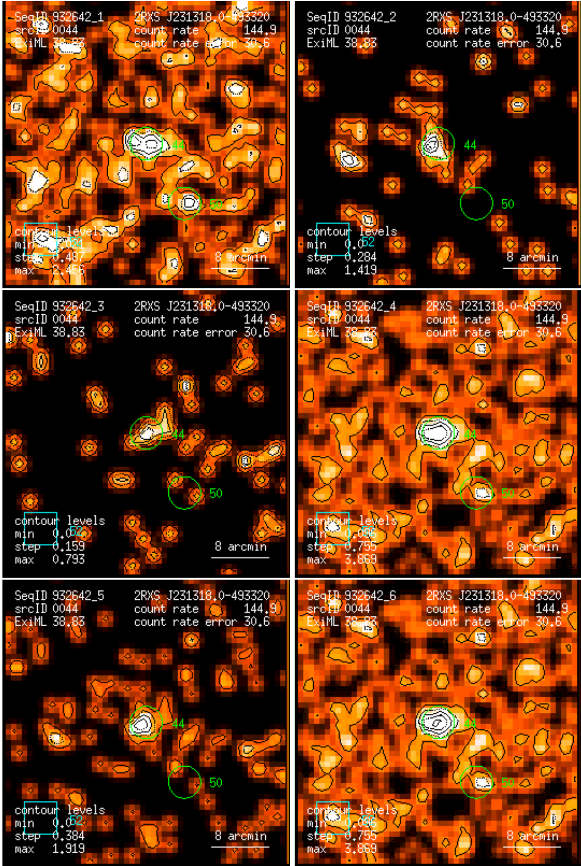
Figure 44: RASS 932642: detection 0044: band rate images, Gaussian filter: (1) PSPC channels 11 – 41, (2) 52 – 90, (3) 91 – 201, (4) 11 – 235, (5) 52 – 201, (6) 11 – 201. Broad band rates in counts/ks. Band rate contour levels in counts/ks/arcmin 2 .
