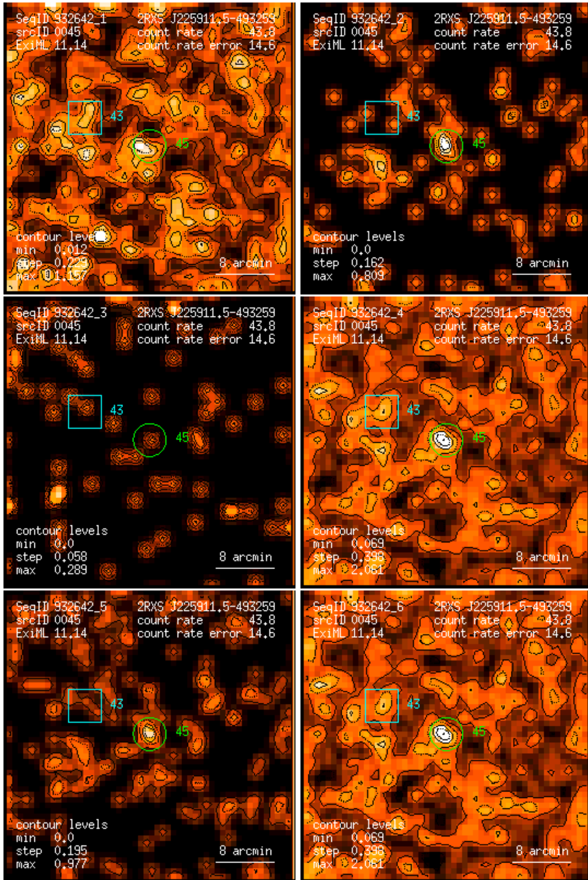
Figure 45: RASS 932642: detection 0045: band rate images, Gaussian filter: (1) PSPC channels 11 – 41, (2) 52 – 90, (3) 91 – 201, (4) 11 – 235, (5) 52 – 201, (6) 11 – 201. Broad band rates in counts/ks. Band rate contour levels in counts/ks/arcmin 2 .
