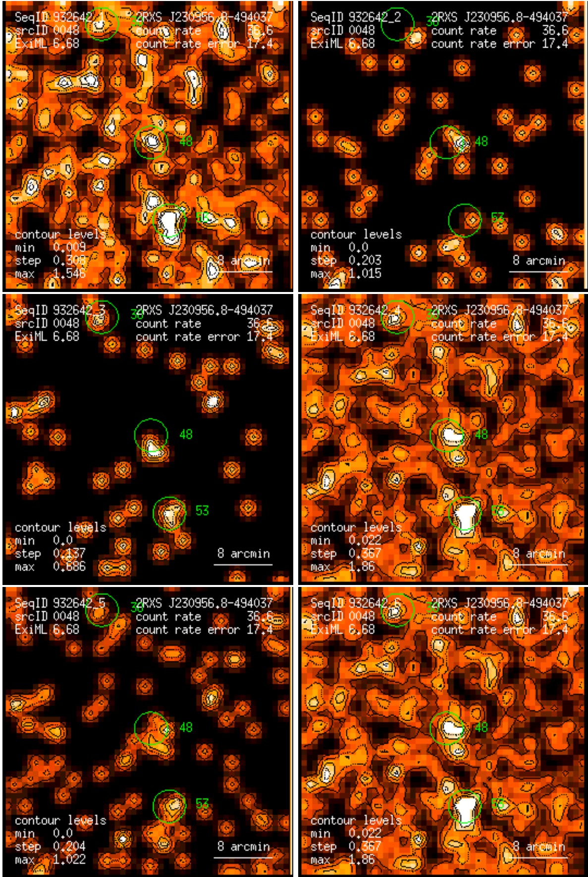
Figure 48: RASS 932642: detection 0048: band rate images, Gaussian filter: (1) PSPC channels 11 – 41, (2) 52 – 90, (3) 91 – 201, (4) 11 – 235, (5) 52 – 201, (6) 11 – 201. Broad band rates in counts/ks. Band rate contour levels in counts/ks/arcmin 2 .
