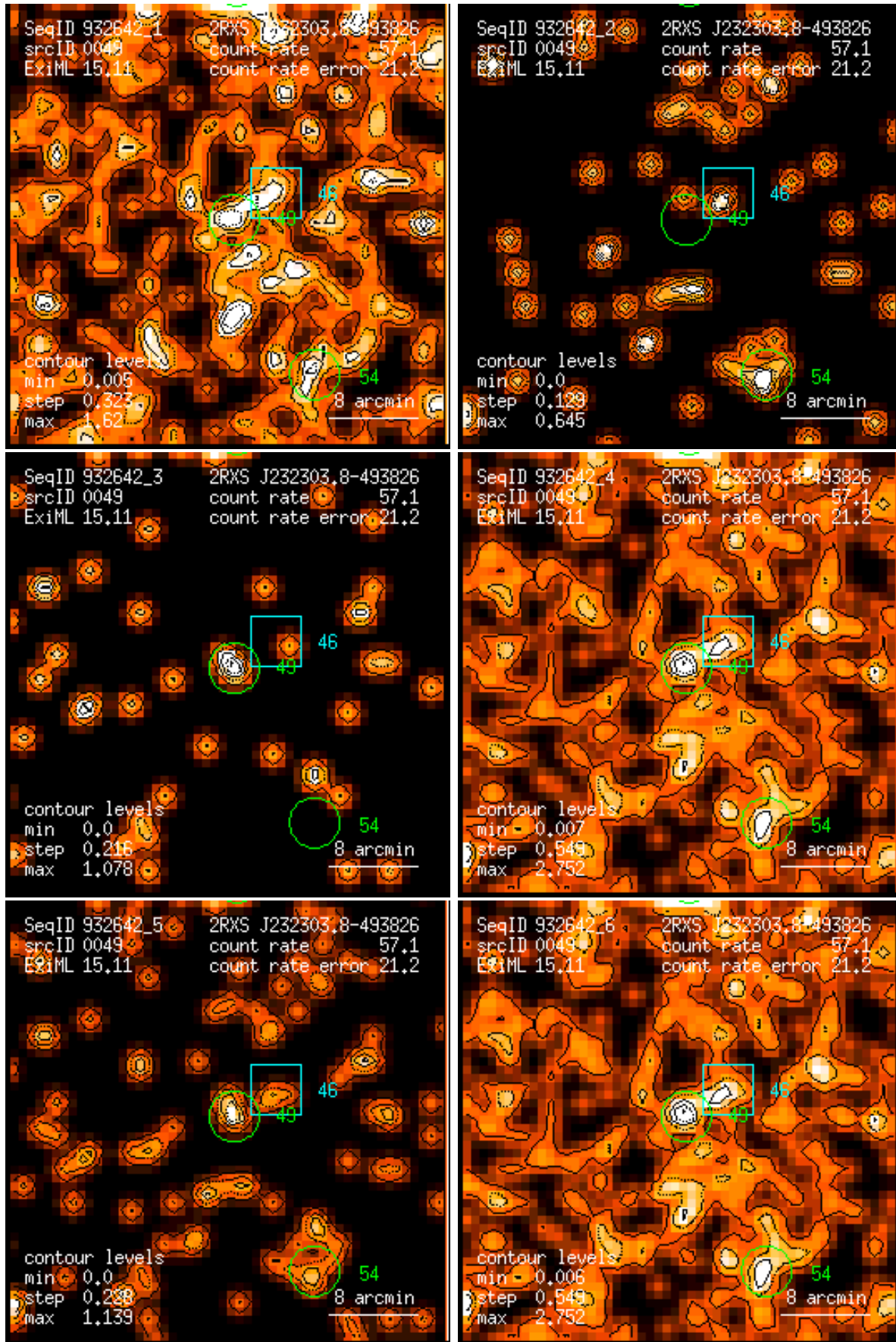
Figure 49: RASS 932642: detection 0049: band rate images, Gaussian filter: (1) PSPC channels 11 – 41, (2) 52 – 90, (3) 91 – 201, (4) 11 – 235, (5) 52 – 201, (6) 11 – 201. Broad band rates in counts/ks. Band rate contour levels in counts/ks/arcmin 2 .
