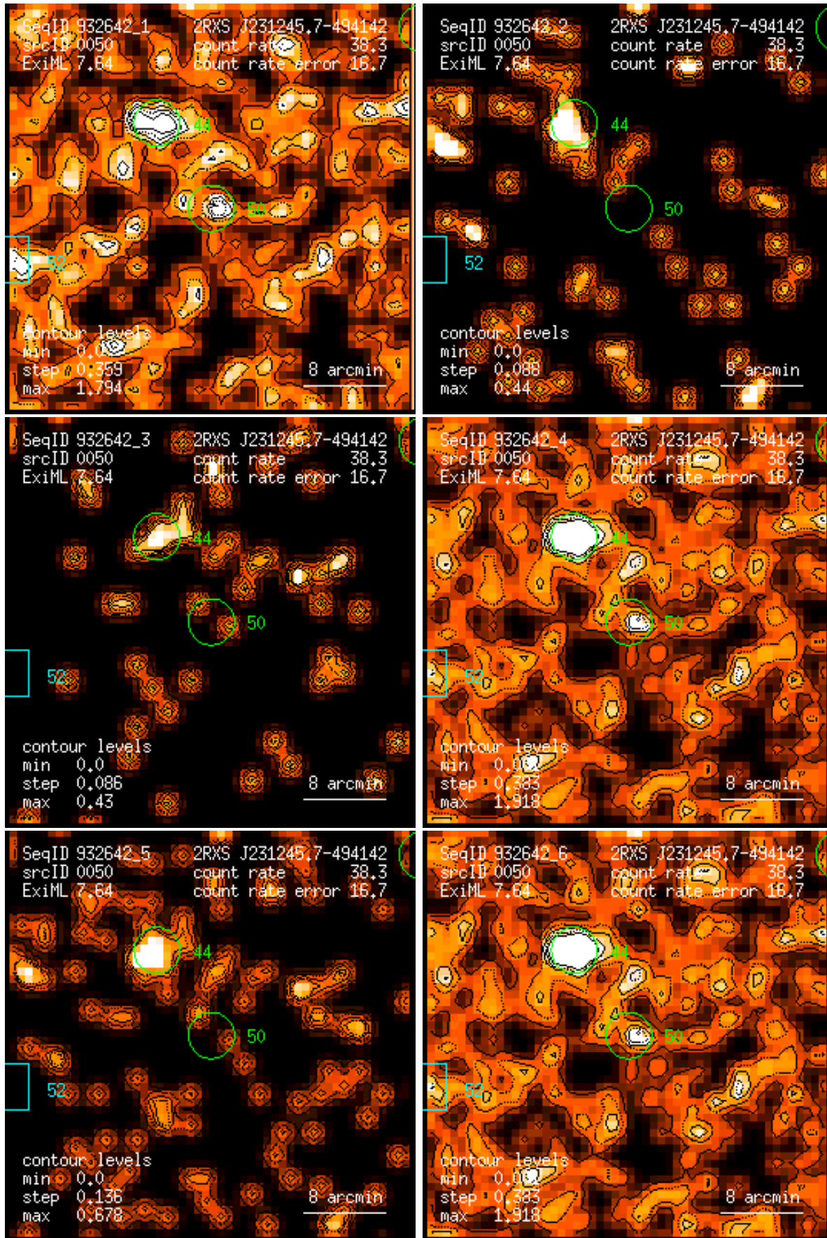
Figure 50: RASS 932642: detection 0050: band rate images, Gaussian filter: (1) PSPC channels 11 – 41, (2) 52 – 90, (3) 91 – 201, (4) 11 – 235, (5) 52 – 201, (6) 11 – 201. Broad band rates in counts/ks. Band rate contour levels in counts/ks/arcmin 2 .
