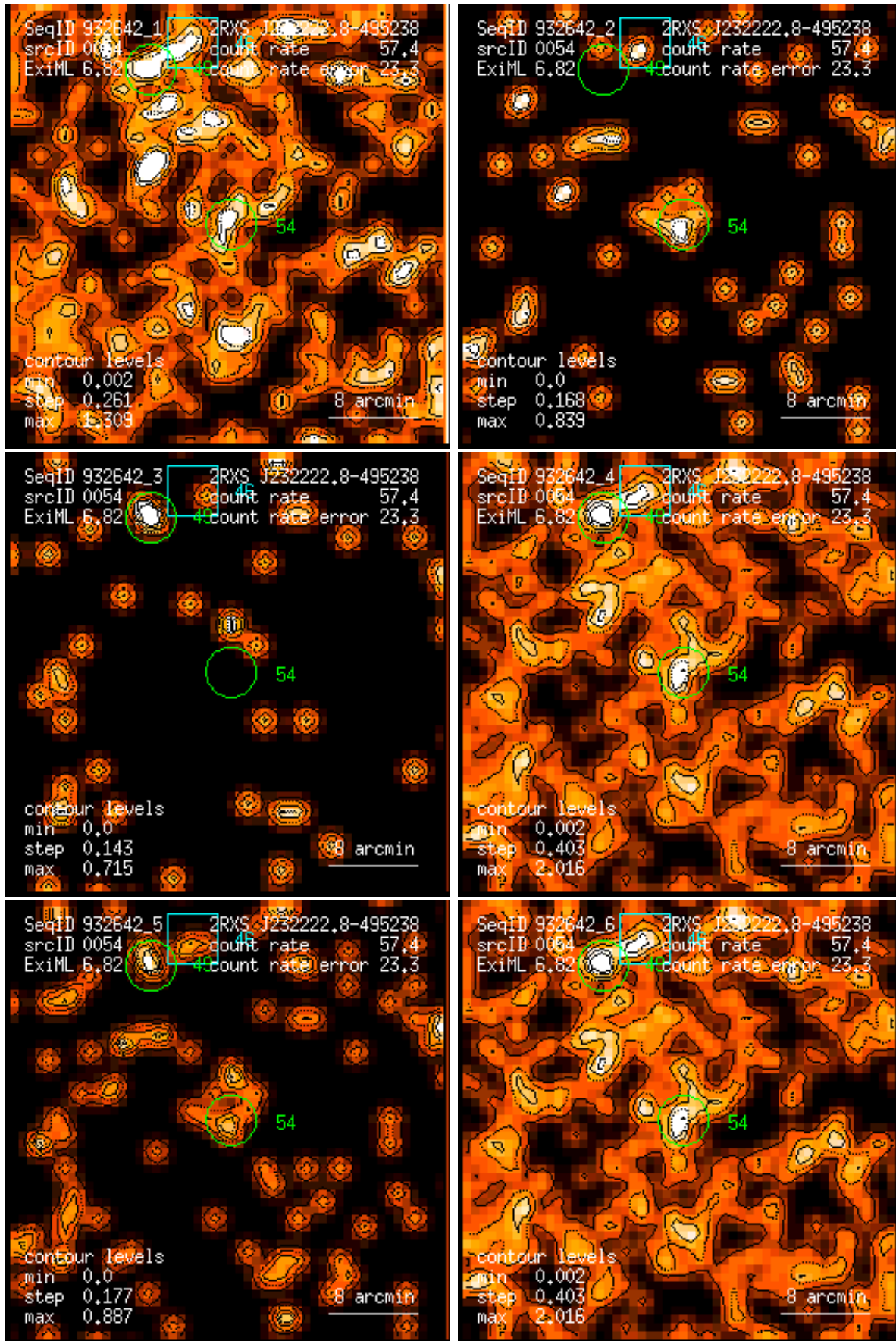
Figure 54: RASS 932642: detection 0054: band rate images, Gaussian filter: (1) PSPC channels 11 – 41, (2) 52 – 90, (3) 91 – 201, (4) 11 – 235, (5) 52 – 201, (6) 11 – 201. Broad band rates in counts/ks. Band rate contour levels in counts/ks/arcmin 2 .
