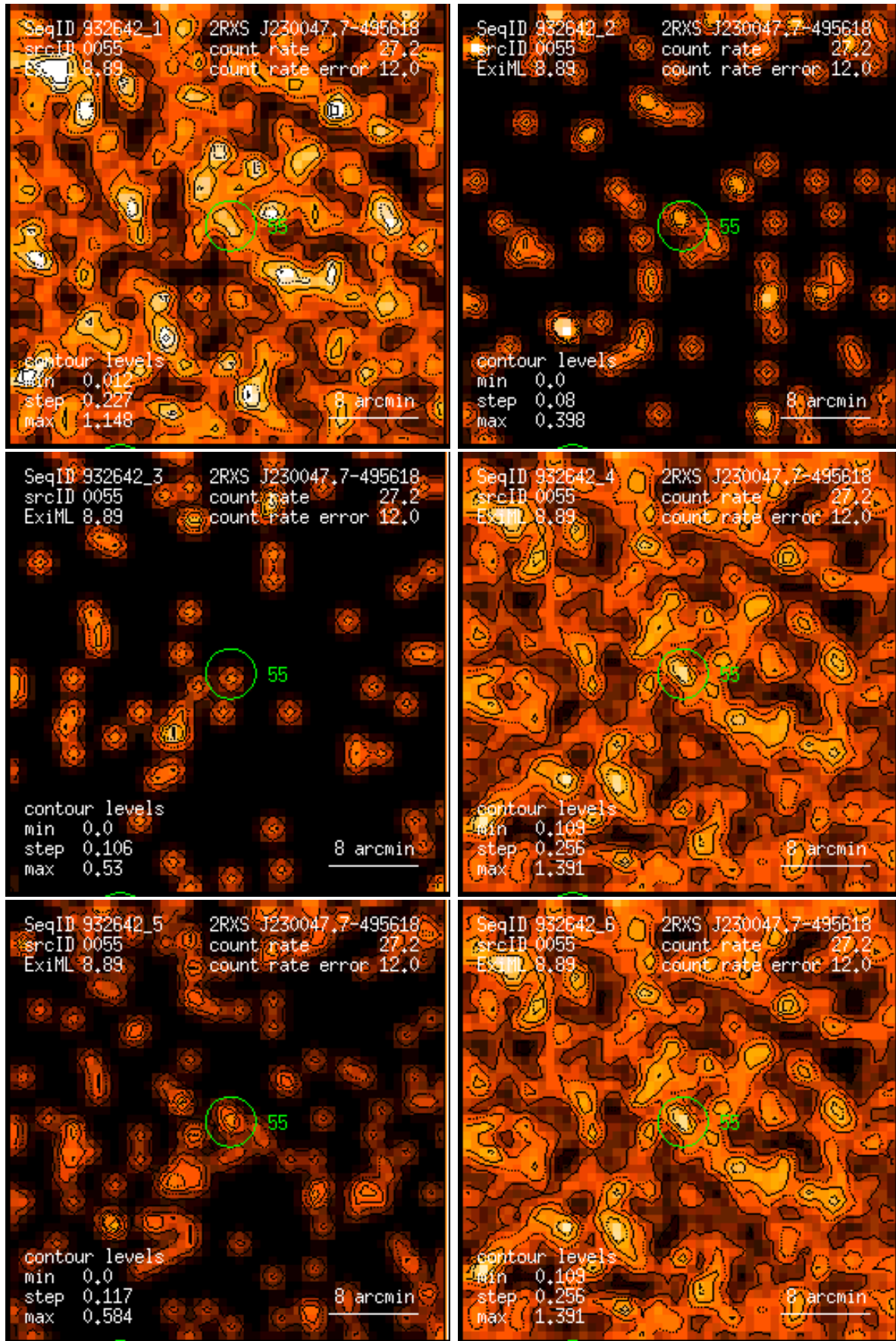
Figure 55: RASS 932642: detection 0055: band rate images, Gaussian filter: (1) PSPC channels 11 – 41, (2) 52 – 90, (3) 91 – 201, (4) 11 – 235, (5) 52 – 201, (6) 11 – 201. Broad band rates in counts/ks. Band rate contour levels in counts/ks/arcmin 2 .
