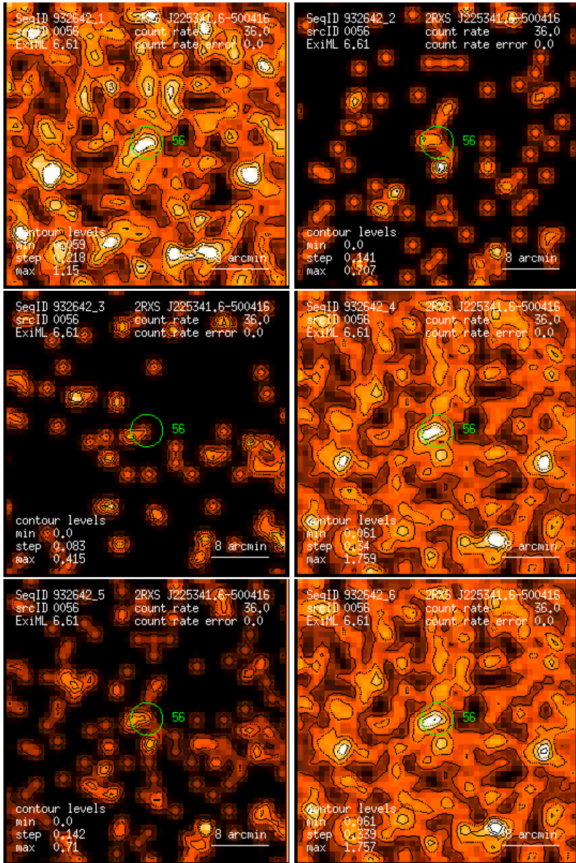
Figure 56: RASS 932642: detection 0056: band rate images, Gaussian filter: (1) PSPC channels 11 – 41, (2) 52 – 90, (3) 91 – 201, (4) 11 – 235, (5) 52 – 201, (6) 11 – 201. Broad band rates in counts/ks. Band rate contour levels in counts/ks/arcmin 2 .
