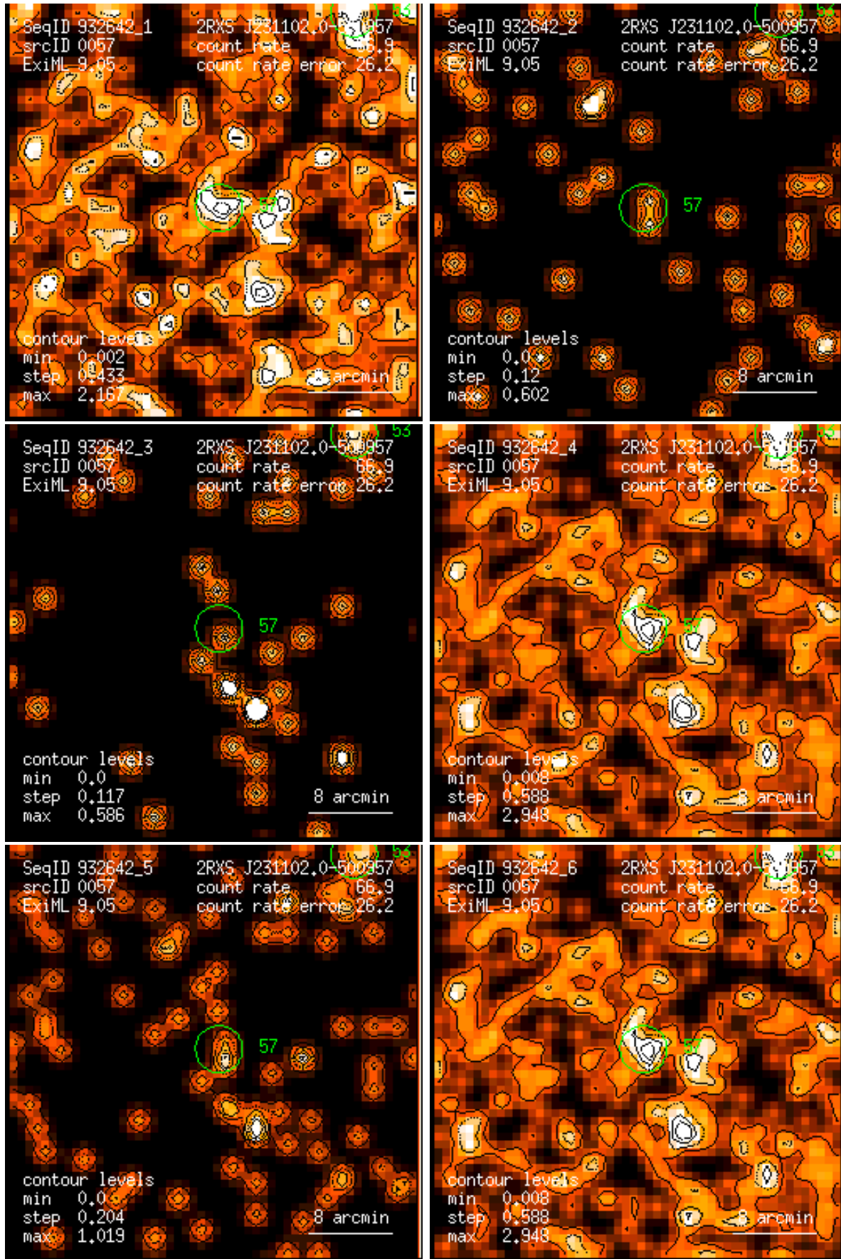
Figure 57: RASS 932642: detection 0057: band rate images, Gaussian filter: (1) PSPC channels 11 – 41, (2) 52 – 90, (3) 91 – 201, (4) 11 – 235, (5) 52 – 201, (6) 11 – 201. Broad band rates in counts/ks. Band rate contour levels in counts/ks/arcmin 2 .
