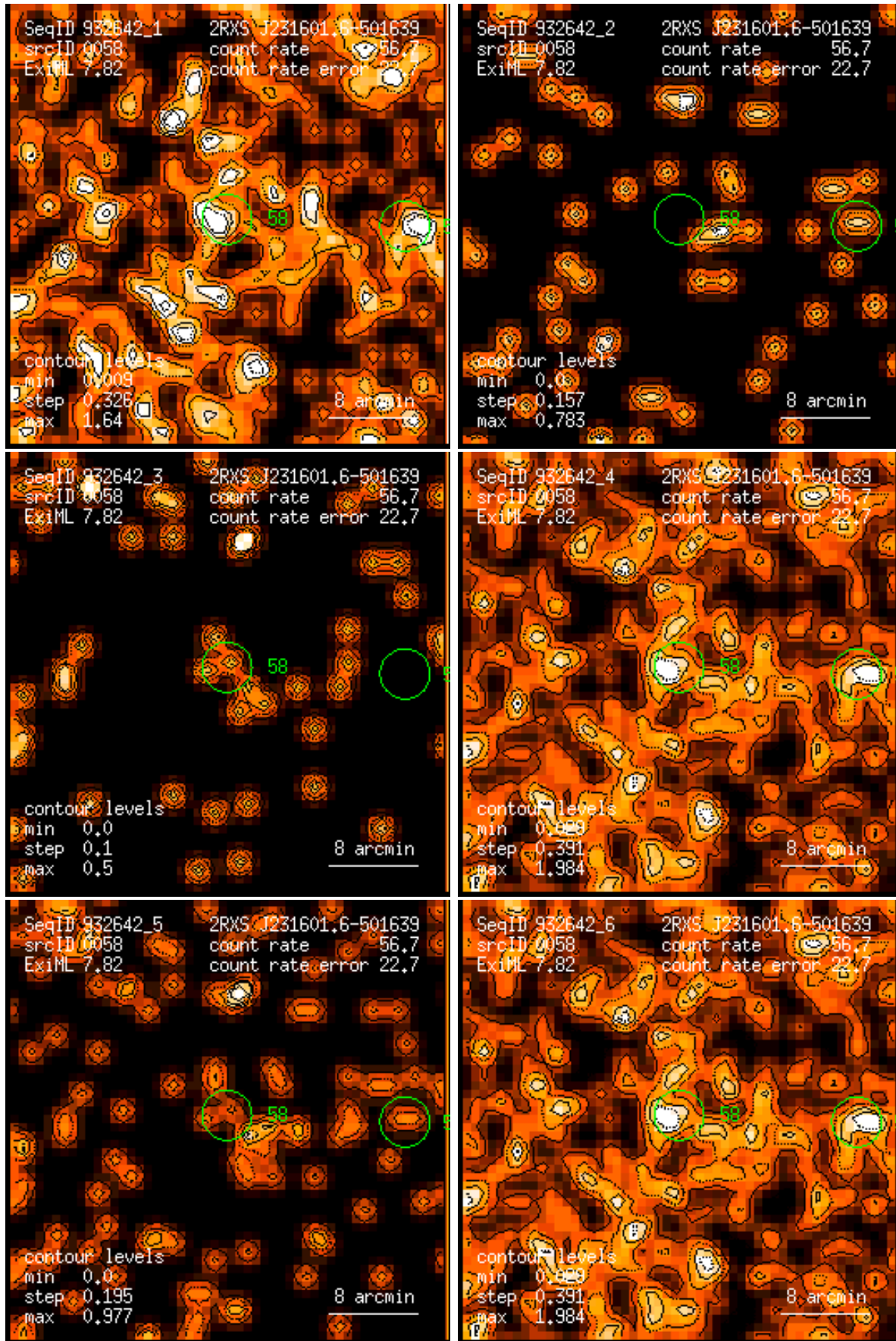
Figure 58: RASS 932642: detection 0058: band rate images, Gaussian filter: (1) PSPC channels 11 – 41, (2) 52 – 90, (3) 91 – 201, (4) 11 – 235, (5) 52 – 201, (6) 11 – 201. Broad band rates in counts/ks. Band rate contour levels in counts/ks/arcmin 2 .
