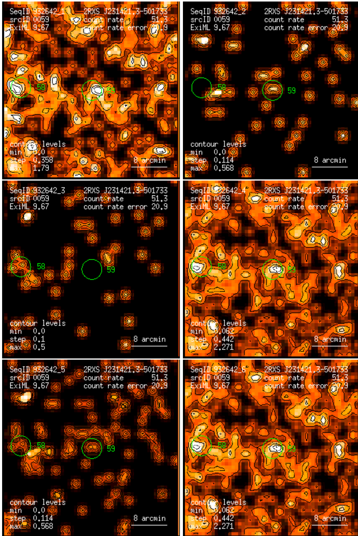
Figure 59: RASS 932642: detection 0059: band rate images, Gaussian filter: (1) PSPC channels 11 – 41, (2) 52 – 90, (3) 91 – 201, (4) 11 – 235, (5) 52 – 201, (6) 11 – 201. Broad band rates in counts/ks. Band rate contour levels in counts/ks/arcmin 2 .
