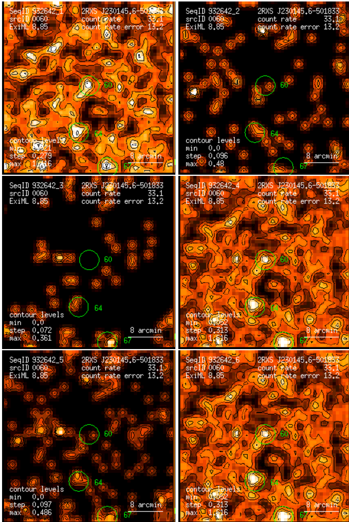
Figure 60: RASS 932642: detection 0060: band rate images, Gaussian filter: (1) PSPC channels 11 – 41, (2) 52 – 90, (3) 91 – 201, (4) 11 – 235, (5) 52 – 201, (6) 11 – 201. Broad band rates in counts/ks. Band rate contour levels in counts/ks/arcmin 2 .
