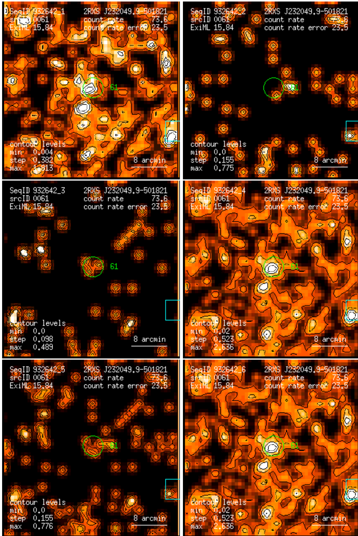
Figure 61: RASS 932642: detection 0061: band rate images, Gaussian filter: (1) PSPC channels 11 – 41, (2) 52 – 90, (3) 91 – 201, (4) 11 – 235, (5) 52 – 201, (6) 11 – 201. Broad band rates in counts/ks. Band rate contour levels in counts/ks/arcmin 2 .
