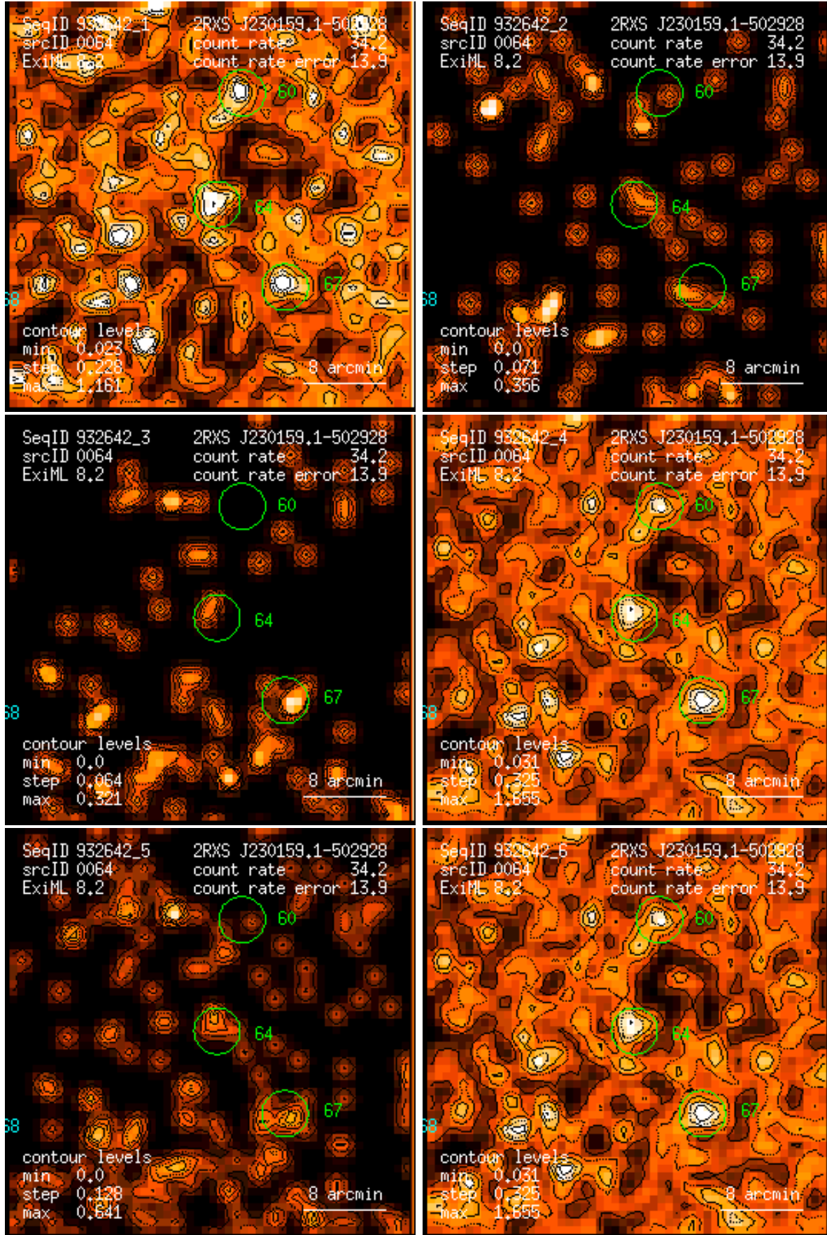
Figure 64: RASS 932642: detection 0064: band rate images, Gaussian filter: (1) PSPC channels 11 – 41, (2) 52 – 90, (3) 91 – 201, (4) 11 – 235, (5) 52 – 201, (6) 11 – 201. Broad band rates in counts/ks. Band rate contour levels in counts/ks/arcmin 2 .
