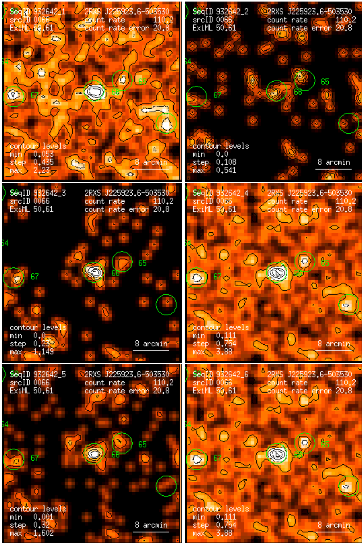
Figure 66: RASS 932642: detection 0066: band rate images, Gaussian filter: (1) PSPC channels 11 – 41, (2) 52 – 90, (3) 91 – 201, (4) 11 – 235, (5) 52 – 201, (6) 11 – 201. Broad band rates in counts/ks. Band rate contour levels in counts/ks/arcmin 2 .
