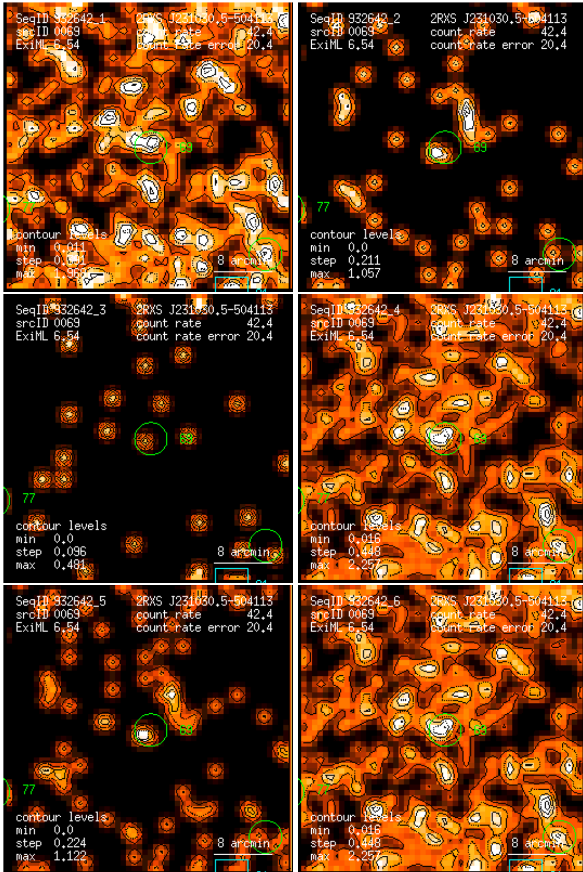
Figure 69: RASS 932642: detection 0069: band rate images, Gaussian filter: (1) PSPC channels 11 – 41, (2) 52 – 90, (3) 91 – 201, (4) 11 – 235, (5) 52 – 201, (6) 11 – 201. Broad band rates in counts/ks. Band rate contour levels in counts/ks/arcmin 2 .
