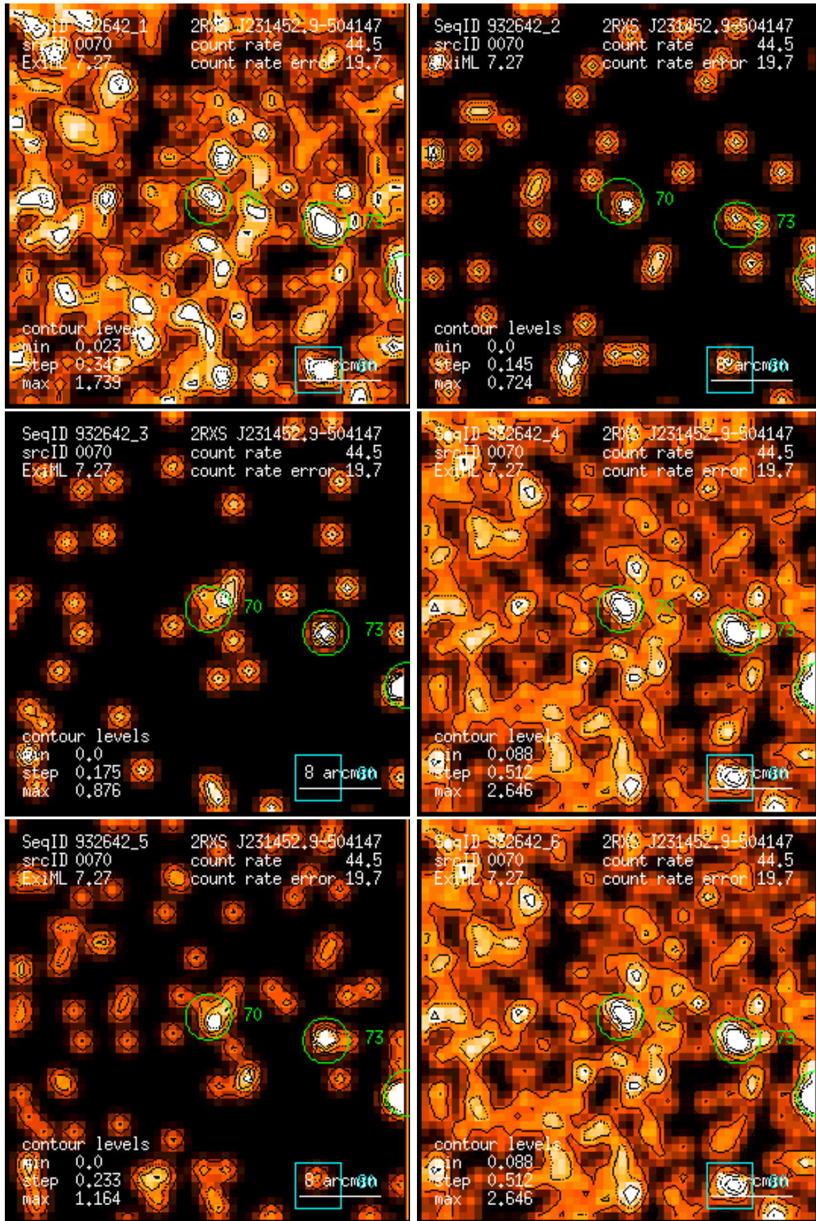
Figure 70: RASS 932642: detection 0070: band rate images, Gaussian filter: (1) PSPC channels 11 – 41, (2) 52 – 90, (3) 91 – 201, (4) 11 – 235, (5) 52 – 201, (6) 11 – 201. Broad band rates in counts/ks. Band rate contour levels in counts/ks/arcmin 2 .
