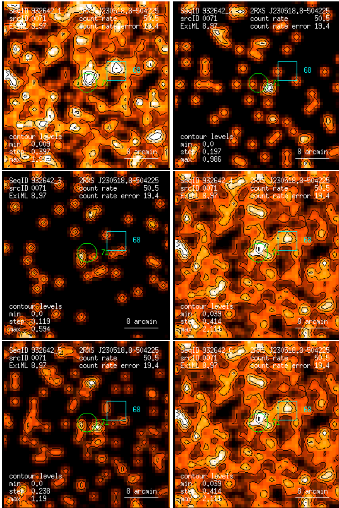
Figure 71: RASS 932642: detection 0071: band rate images, Gaussian filter: (1) PSPC channels 11 – 41, (2) 52 – 90, (3) 91 – 201, (4) 11 – 235, (5) 52 – 201, (6) 11 – 201. Broad band rates in counts/ks. Band rate contour levels in counts/ks/arcmin 2 .
