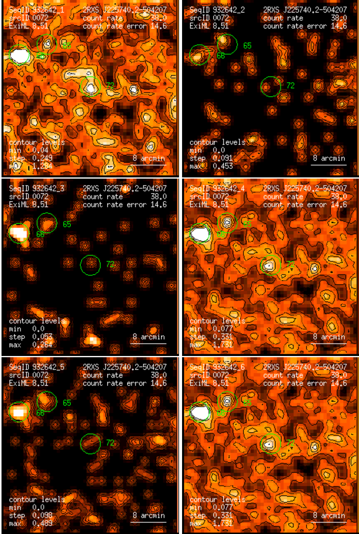
Figure 72: RASS 932642: detection 0072: band rate images, Gaussian filter: (1) PSPC channels 11 – 41, (2) 52 – 90, (3) 91 – 201, (4) 11 – 235, (5) 52 – 201, (6) 11 – 201. Broad band rates in counts/ks. Band rate contour levels in counts/ks/arcmin 2 .
