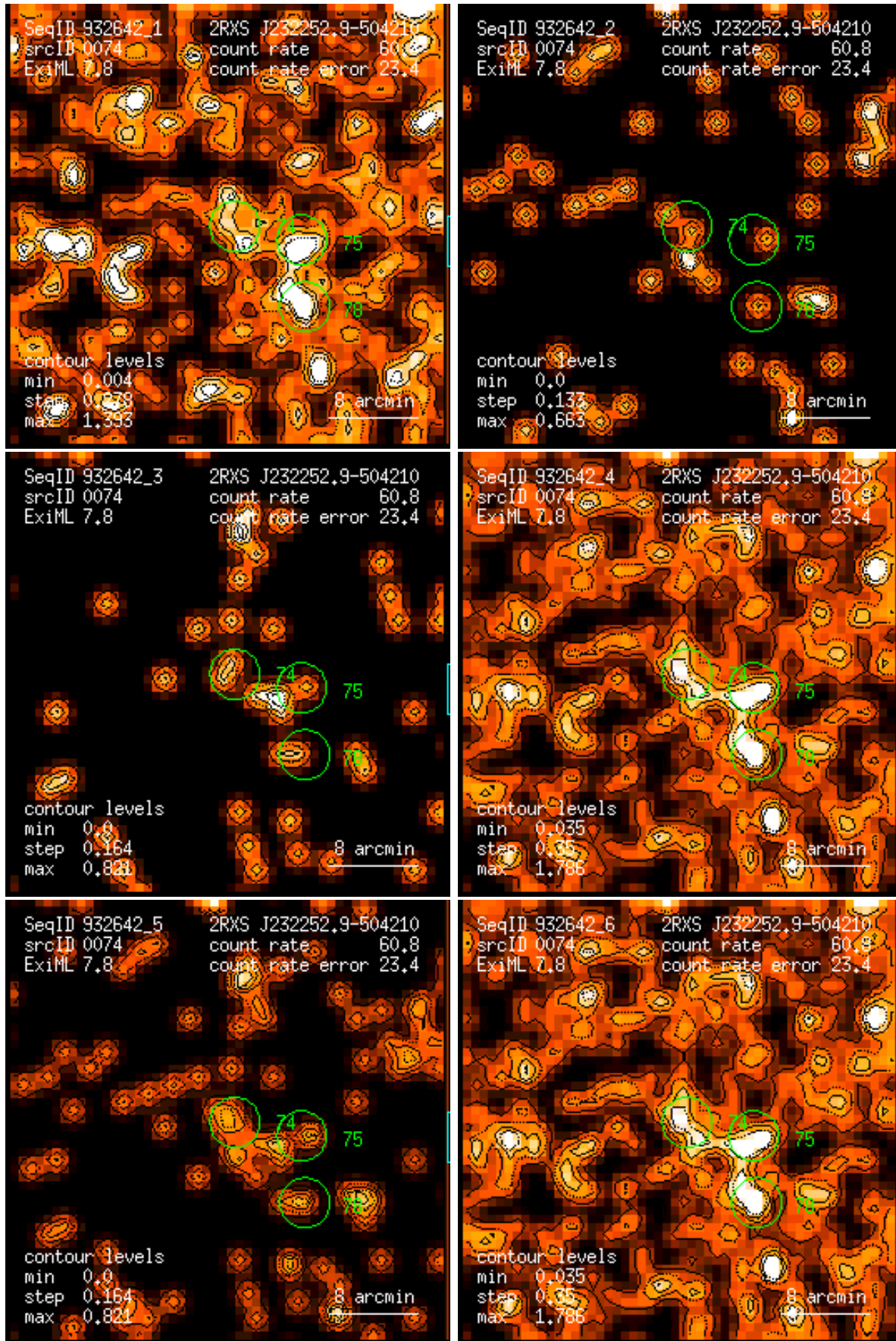
Figure 74: RASS 932642: detection 0074: band rate images, Gaussian filter: (1) PSPC channels 11 – 41, (2) 52 – 90, (3) 91 – 201, (4) 11 – 235, (5) 52 – 201, (6) 11 – 201. Broad band rates in counts/ks. Band rate contour levels in counts/ks/arcmin 2 .
