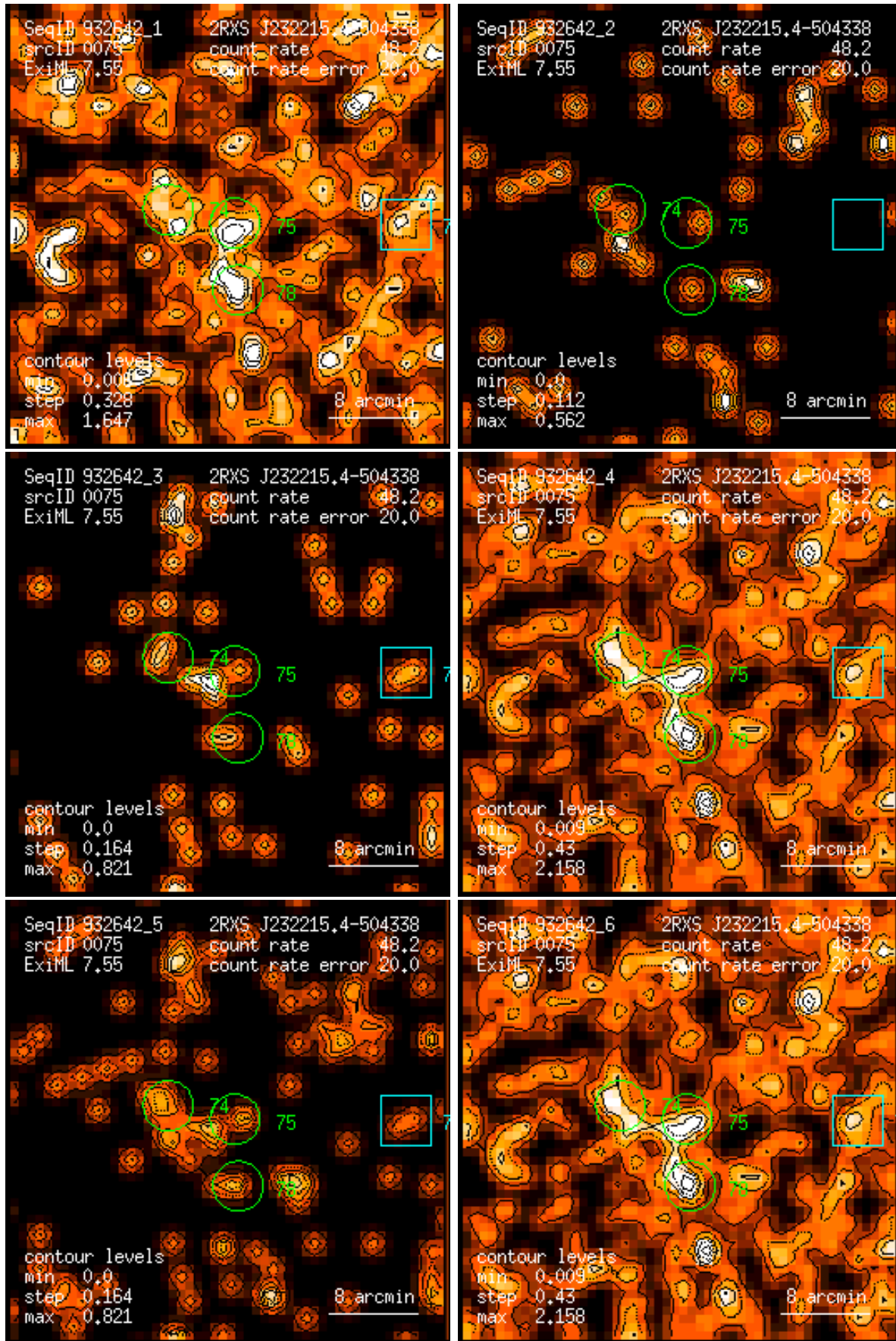
Figure 75: RASS 932642: detection 0075: band rate images, Gaussian filter: (1) PSPC channels 11 – 41, (2) 52 – 90, (3) 91 – 201, (4) 11 – 235, (5) 52 – 201, (6) 11 – 201. Broad band rates in counts/ks. Band rate contour levels in counts/ks/arcmin 2 .
