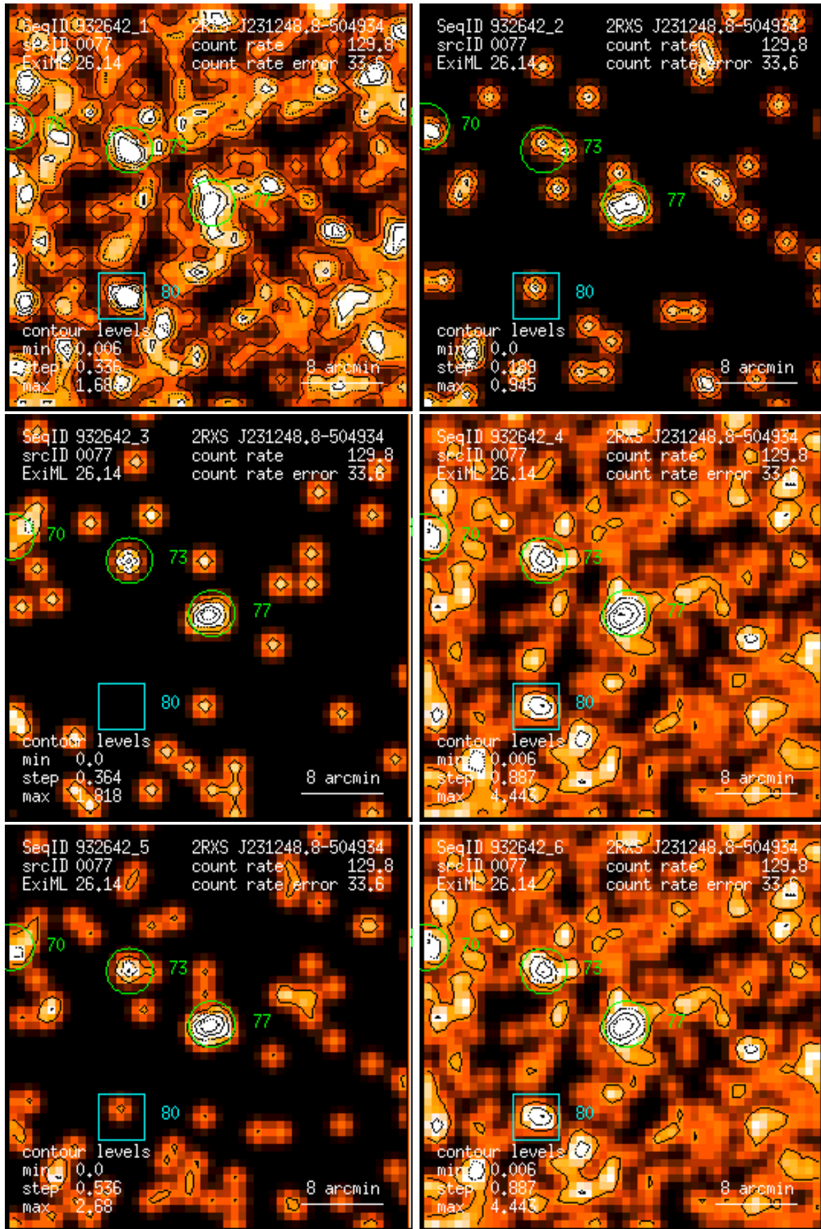
Figure 77: RASS 932642: detection 0077: band rate images, Gaussian filter: (1) PSPC channels 11 – 41, (2) 52 – 90, (3) 91 – 201, (4) 11 – 235, (5) 52 – 201, (6) 11 – 201. Broad band rates in counts/ks. Band rate contour levels in counts/ks/arcmin 2 .
