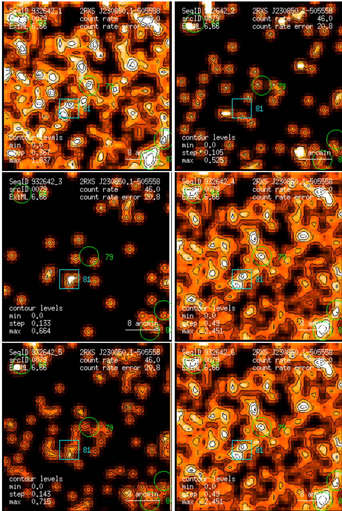
Figure 79: RASS 932642: detection 0079: band rate images, Gaussian filter: (1) PSPC channels 11 – 41, (2) 52 – 90, (3) 91 – 201, (4) 11 – 235, (5) 52 – 201, (6) 11 – 201. Broad band rates in counts/ks. Band rate contour levels in counts/ks/arcmin 2 .
