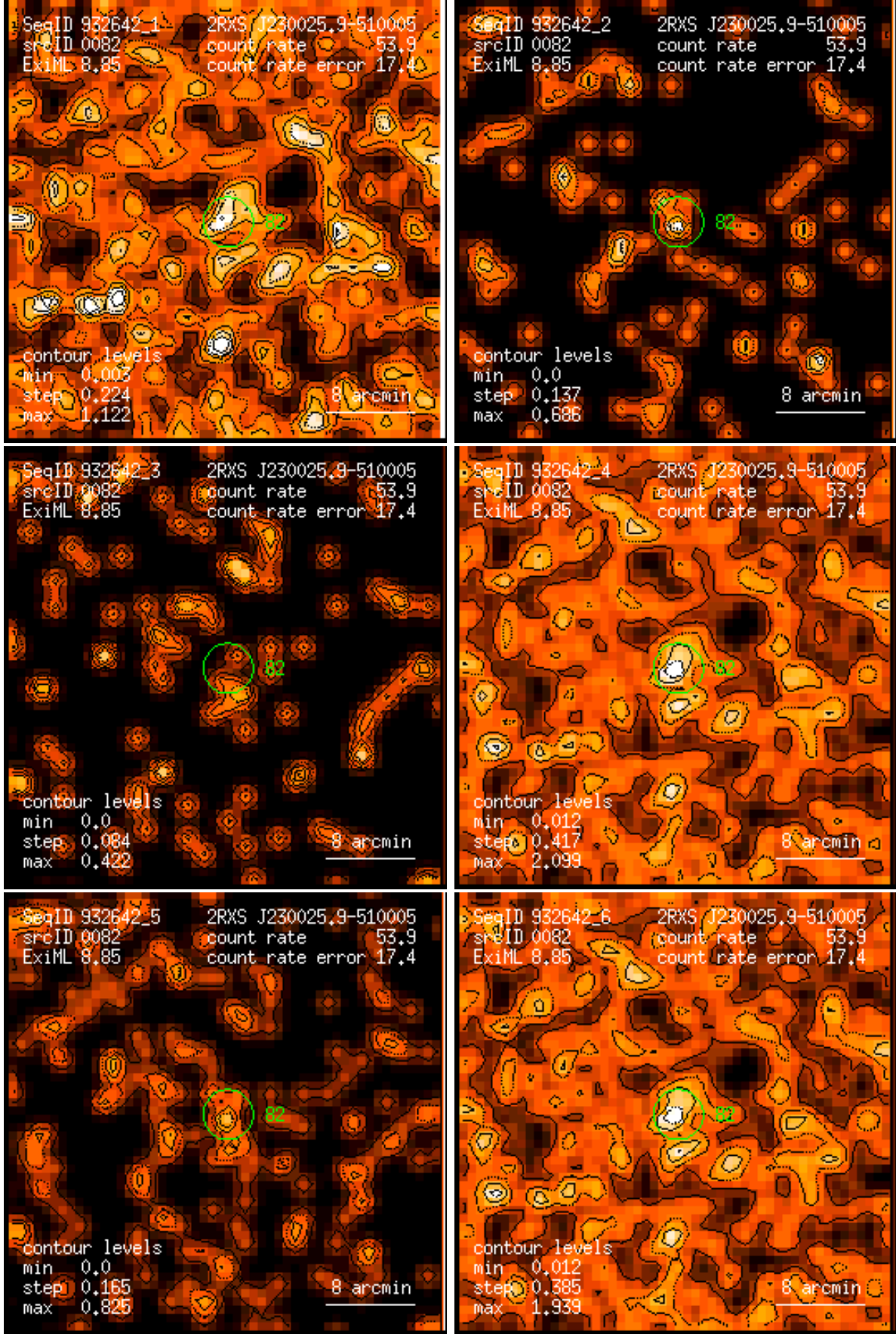
Figure 82: RASS 932642: detection 0082: band rate images, Gaussian filter: (1) PSPC channels 11 – 41, (2) 52 – 90, (3) 91 – 201, (4) 11 – 235, (5) 52 – 201, (6) 11 – 201. Broad band rates in counts/ks. Band rate contour levels in counts/ks/arcmin 2 .
