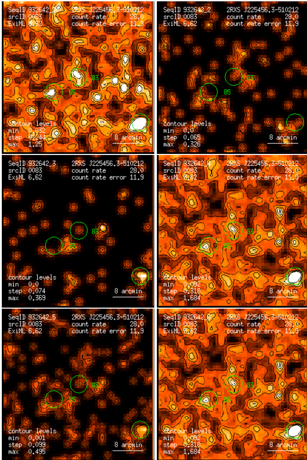
Figure 83: RASS 932642: detection 0083: band rate images, Gaussian filter: (1) PSPC channels 11 – 41, (2) 52 – 90, (3) 91 – 201, (4) 11 – 235, (5) 52 – 201, (6) 11 – 201. Broad band rates in counts/ks. Band rate contour levels in counts/ks/arcmin 2 .
