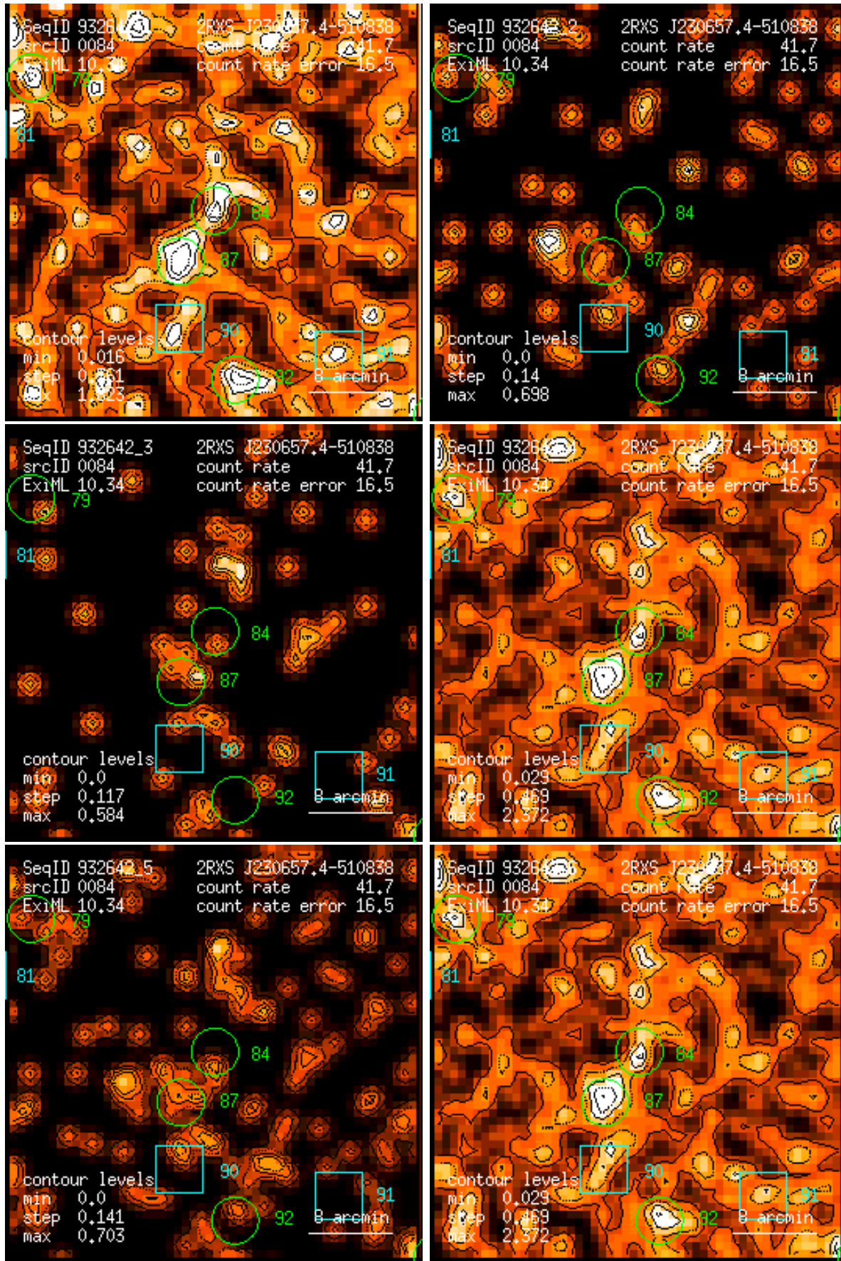
Figure 84: RASS 932642: detection 0084: band rate images, Gaussian filter: (1) PSPC channels 11 – 41, (2) 52 – 90, (3) 91 – 201, (4) 11 – 235, (5) 52 – 201, (6) 11 – 201. Broad band rates in counts/ks. Band rate contour levels in counts/ks/arcmin 2 .
