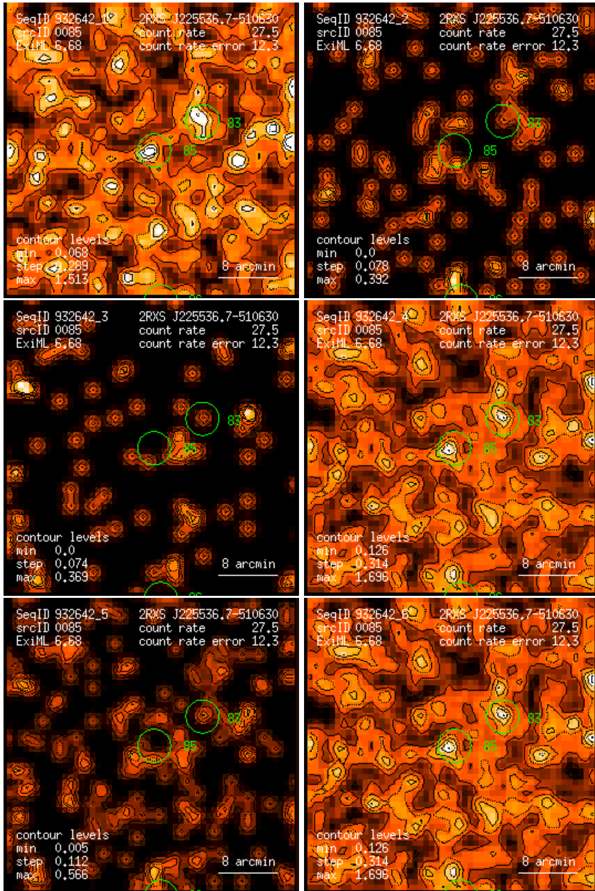
Figure 85: RASS 932642: detection 0085: band rate images, Gaussian filter: (1) PSPC channels 11 – 41, (2) 52 – 90, (3) 91 – 201, (4) 11 – 235, (5) 52 – 201, (6) 11 – 201. Broad band rates in counts/ks. Band rate contour levels in counts/ks/arcmin 2 .
