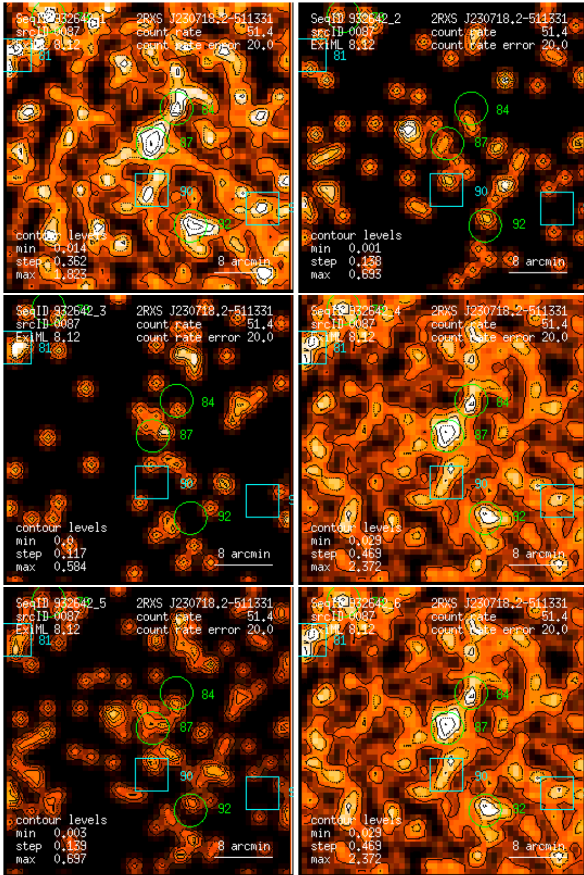
Figure 87: RASS 932642: detection 0087: band rate images, Gaussian filter: (1) PSPC channels 11 – 41, (2) 52 – 90, (3) 91 – 201, (4) 11 – 235, (5) 52 – 201, (6) 11 – 201. Broad band rates in counts/ks. Band rate contour levels in counts/ks/arcmin 2 .
