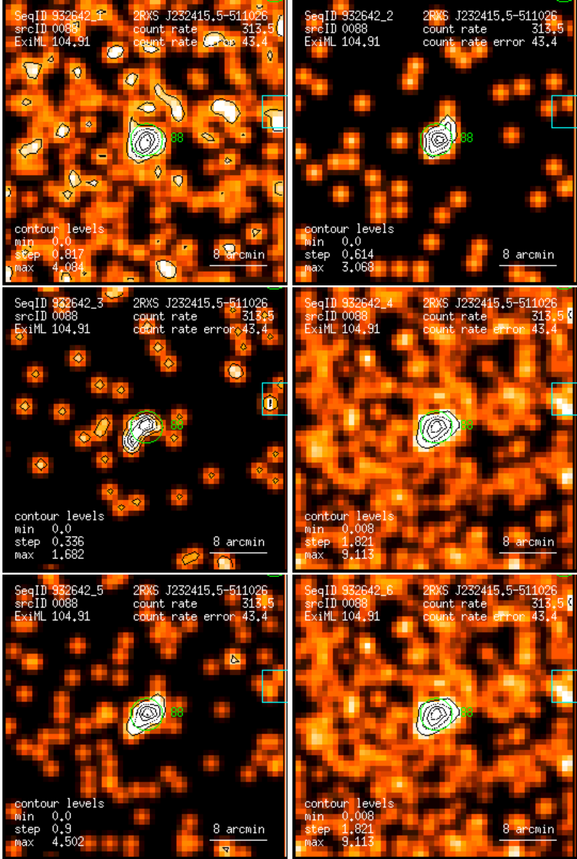
Figure 88: RASS 932642: detection 0088: band rate images, Gaussian filter: (1) PSPC channels 11 – 41, (2) 52 – 90, (3) 91 – 201, (4) 11 – 235, (5) 52 – 201, (6) 11 – 201. Broad band rates in counts/ks. Band rate contour levels in counts/ks/arcmin 2 .
