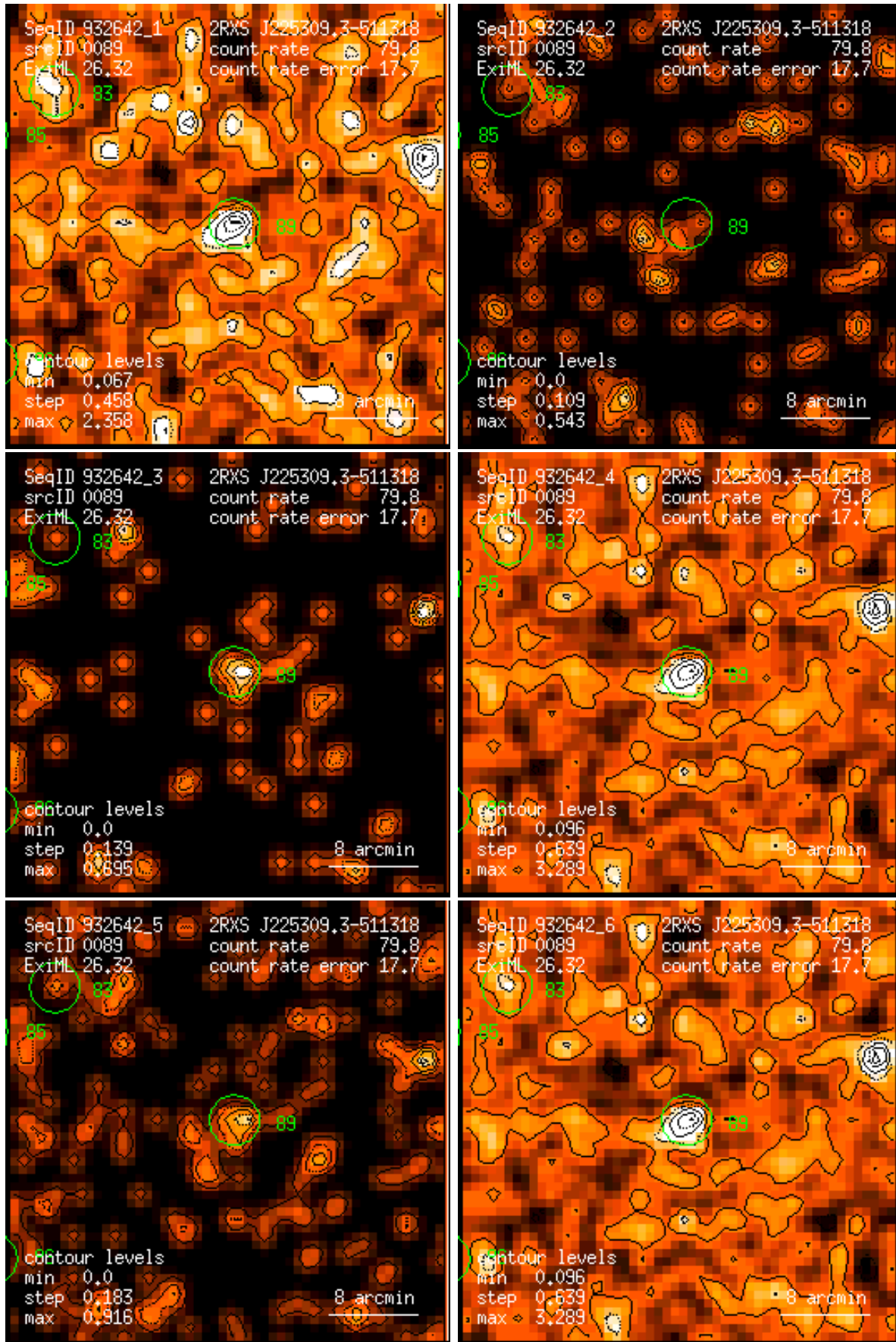
Figure 89: RASS 932642: detection 0089: band rate images, Gaussian filter: (1) PSPC channels 11 – 41, (2) 52 – 90, (3) 91 – 201, (4) 11 – 235, (5) 52 – 201, (6) 11 – 201. Broad band rates in counts/ks. Band rate contour levels in counts/ks/arcmin 2 .
