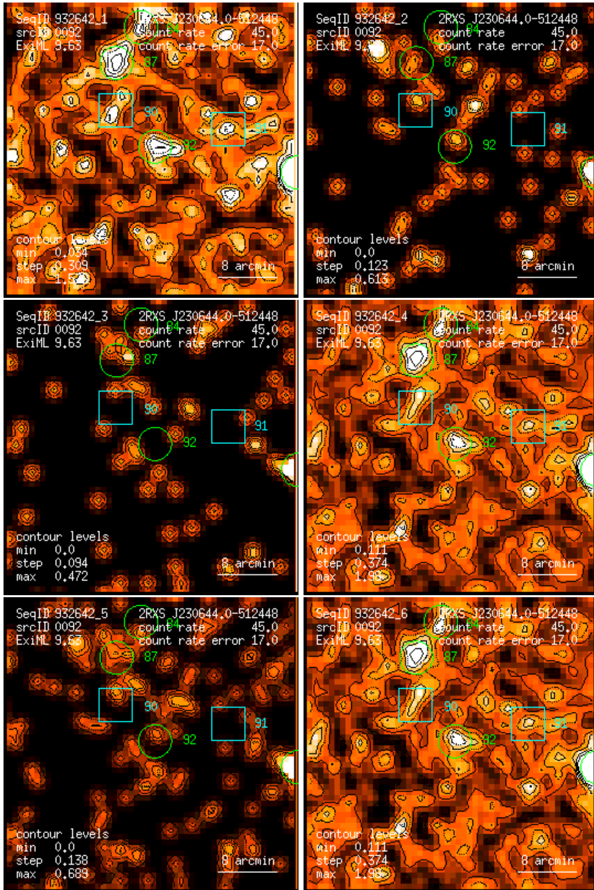
Figure 92: RASS 932642: detection 0092: band rate images, Gaussian filter: (1) PSPC channels 11 – 41, (2) 52 – 90, (3) 91 – 201, (4) 11 – 235, (5) 52 – 201, (6) 11 – 201. Broad band rates in counts/ks. Band rate contour levels in counts/ks/arcmin 2 .
