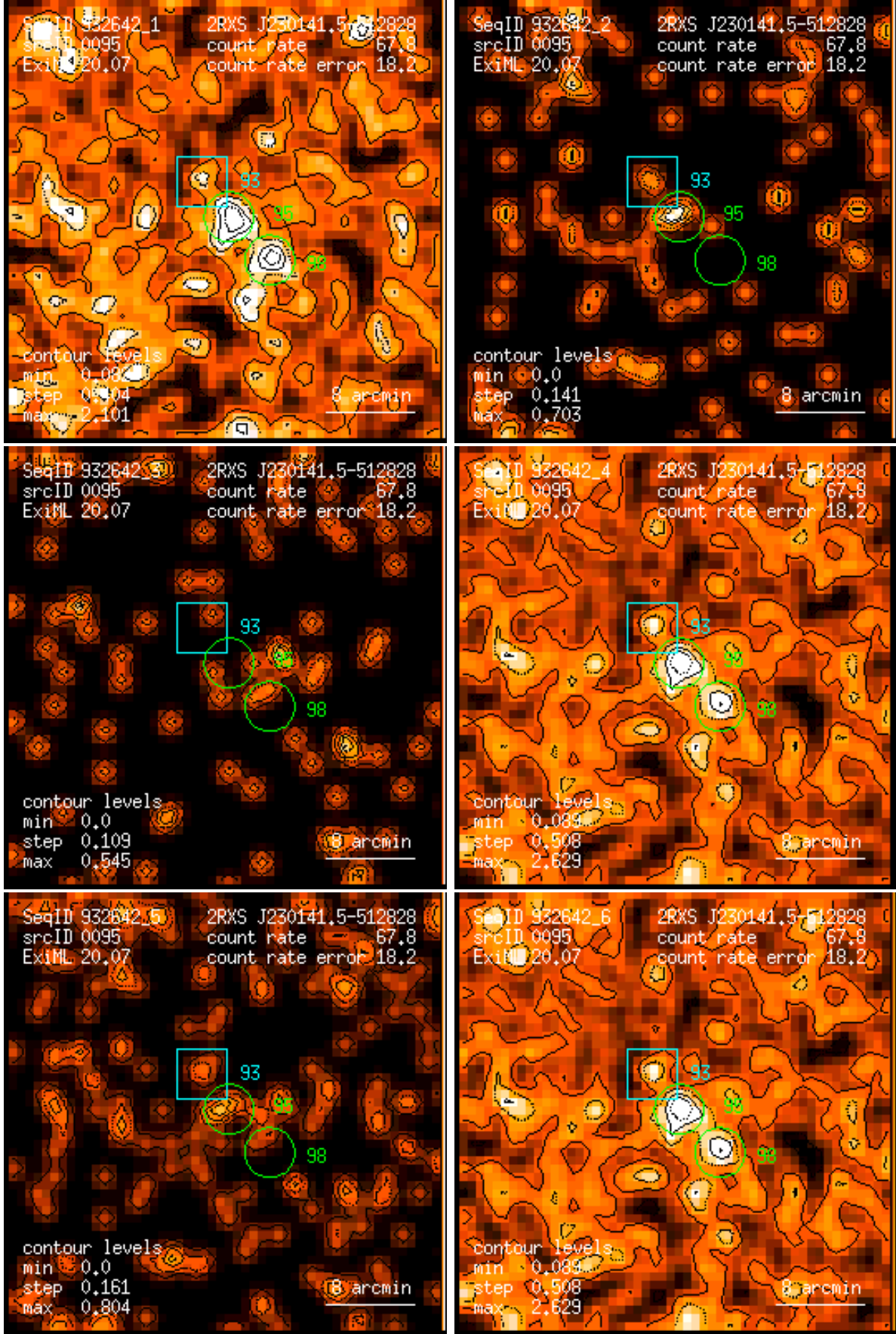
Figure 95: RASS 932642: detection 0095: band rate images, Gaussian filter: (1) PSPC channels 11 – 41, (2) 52 – 90, (3) 91 – 201, (4) 11 – 235, (5) 52 – 201, (6) 11 – 201. Broad band rates in counts/ks. Band rate contour levels in counts/ks/arcmin 2 .
