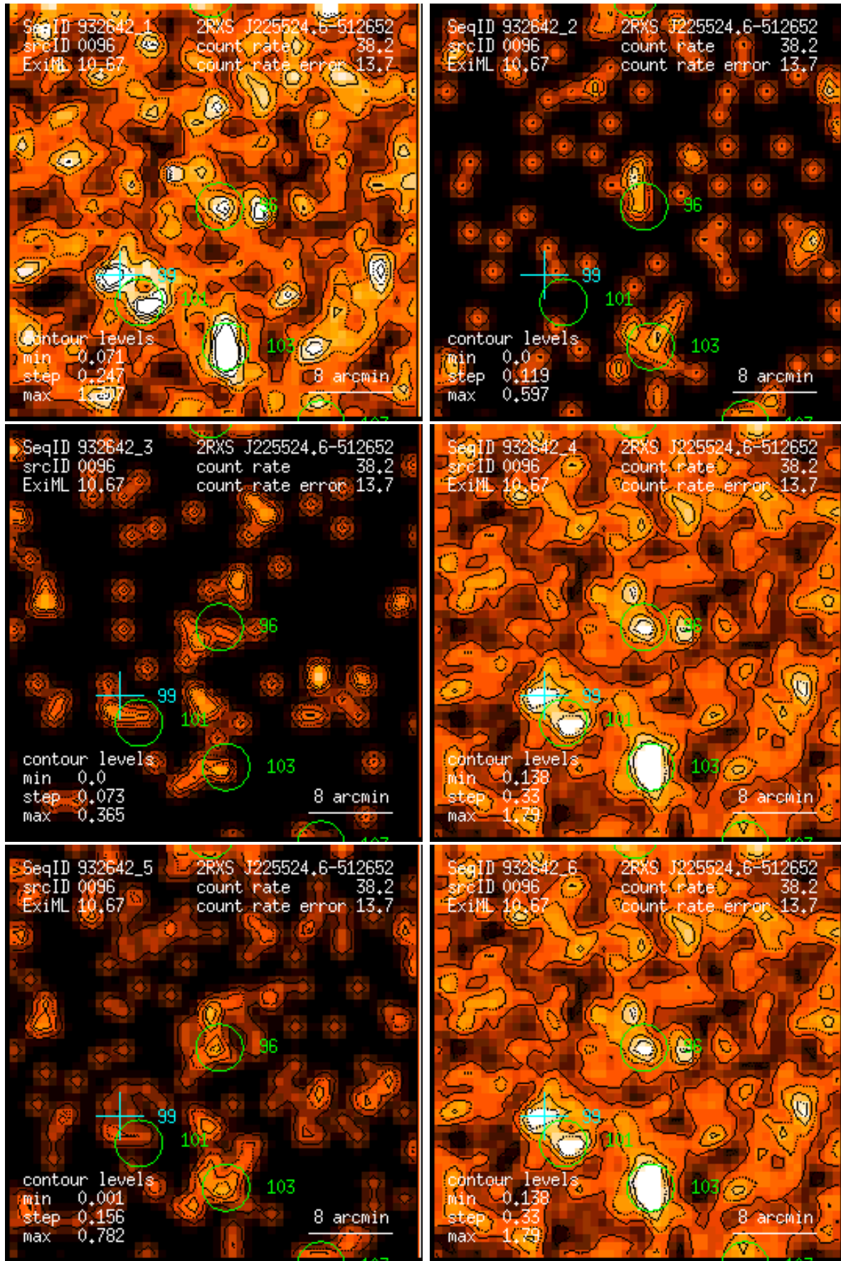
Figure 96: RASS 932642: detection 0096: band rate images, Gaussian filter: (1) PSPC channels 11 – 41, (2) 52 – 90, (3) 91 – 201, (4) 11 – 235, (5) 52 – 201, (6) 11 – 201. Broad band rates in counts/ks. Band rate contour levels in counts/ks/arcmin 2 .
