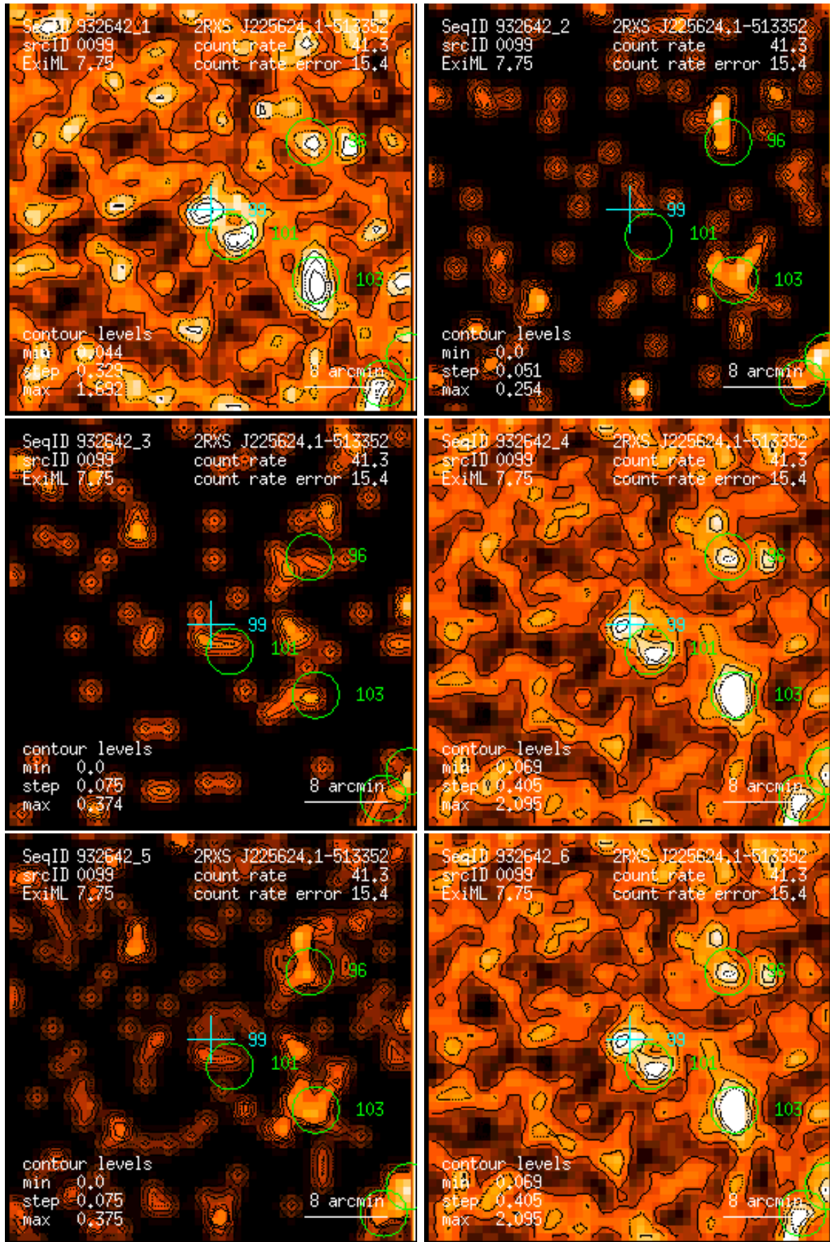
Figure 99: RASS 932642: detection 0099: band rate images, Gaussian filter: (1) PSPC channels 11 – 41, (2) 52 – 90, (3) 91 – 201, (4) 11 – 235, (5) 52 – 201, (6) 11 – 201. Broad band rates in counts/ks. Band rate contour levels in counts/ks/arcmin 2 .
