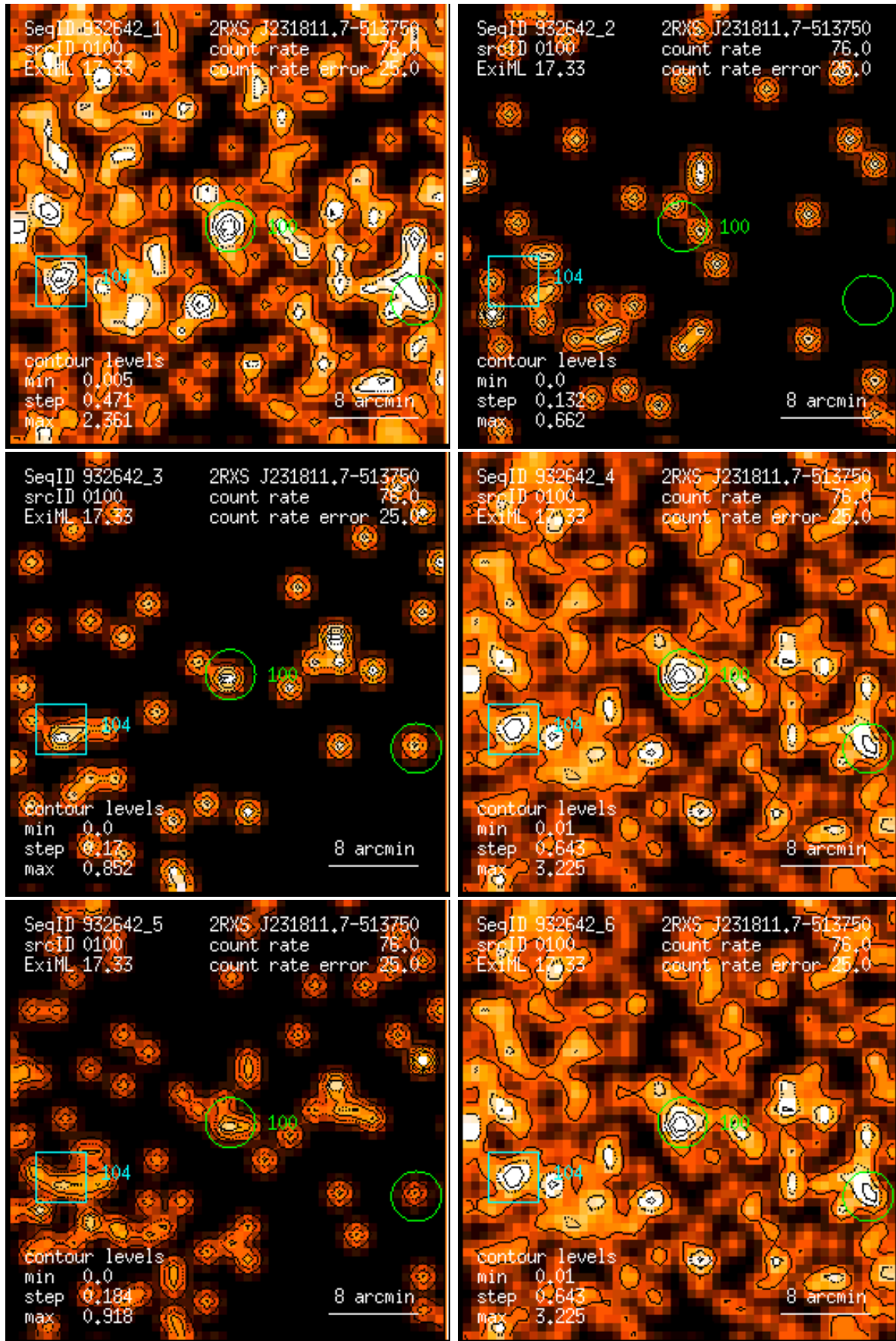
Figure 100: RASS 932642: detection 0100: band rate images, Gaussian filter: (1) PSPC channels 11 – 41, (2) 52 – 90, (3) 91 – 201, (4) 11 – 235, (5) 52 – 201, (6) 11 – 201. Broad band rates in counts/ks. Band rate contour levels in counts/ks/arcmin 2 .
