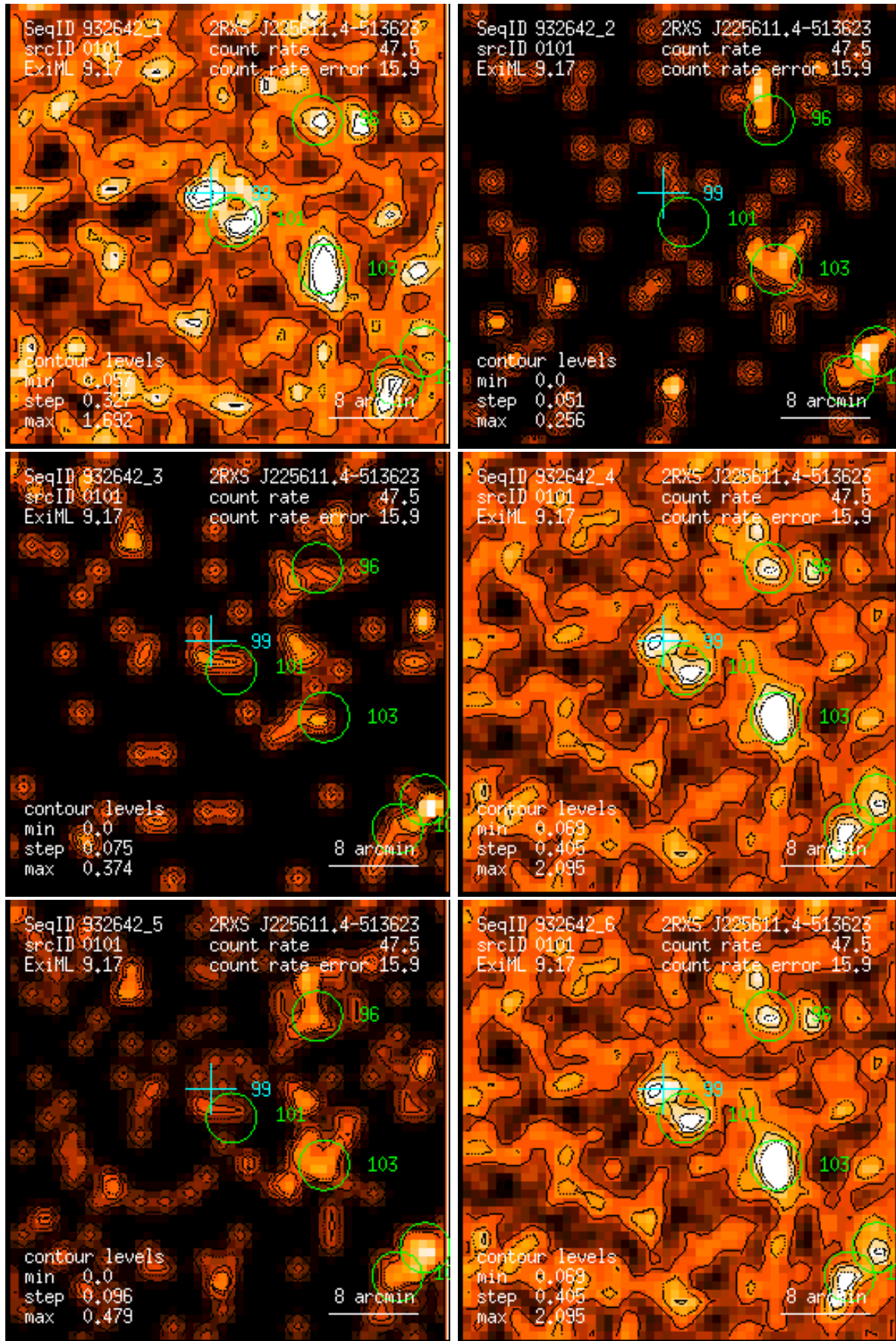
Figure 101: RASS 932642: detection 0101: band rate images, Gaussian filter: (1) PSPC channels 11 – 41, (2) 52 – 90, (3) 91 – 201, (4) 11 – 235, (5) 52 – 201, (6) 11 – 201. Broad band rates in counts/ks. Band rate contour levels in counts/ks/arcmin 2 .
