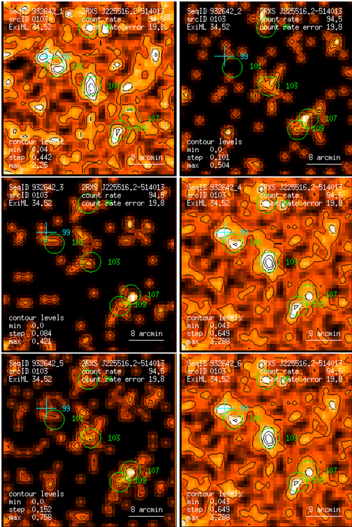
Figure 103: RASS 932642: detection 0103: band rate images, Gaussian filter: (1) PSPC channels 11 – 41, (2) 52 – 90, (3) 91 – 201, (4) 11 – 235, (5) 52 – 201, (6) 11 – 201. Broad band rates in counts/ks. Band rate contour levels in counts/ks/arcmin 2 .
