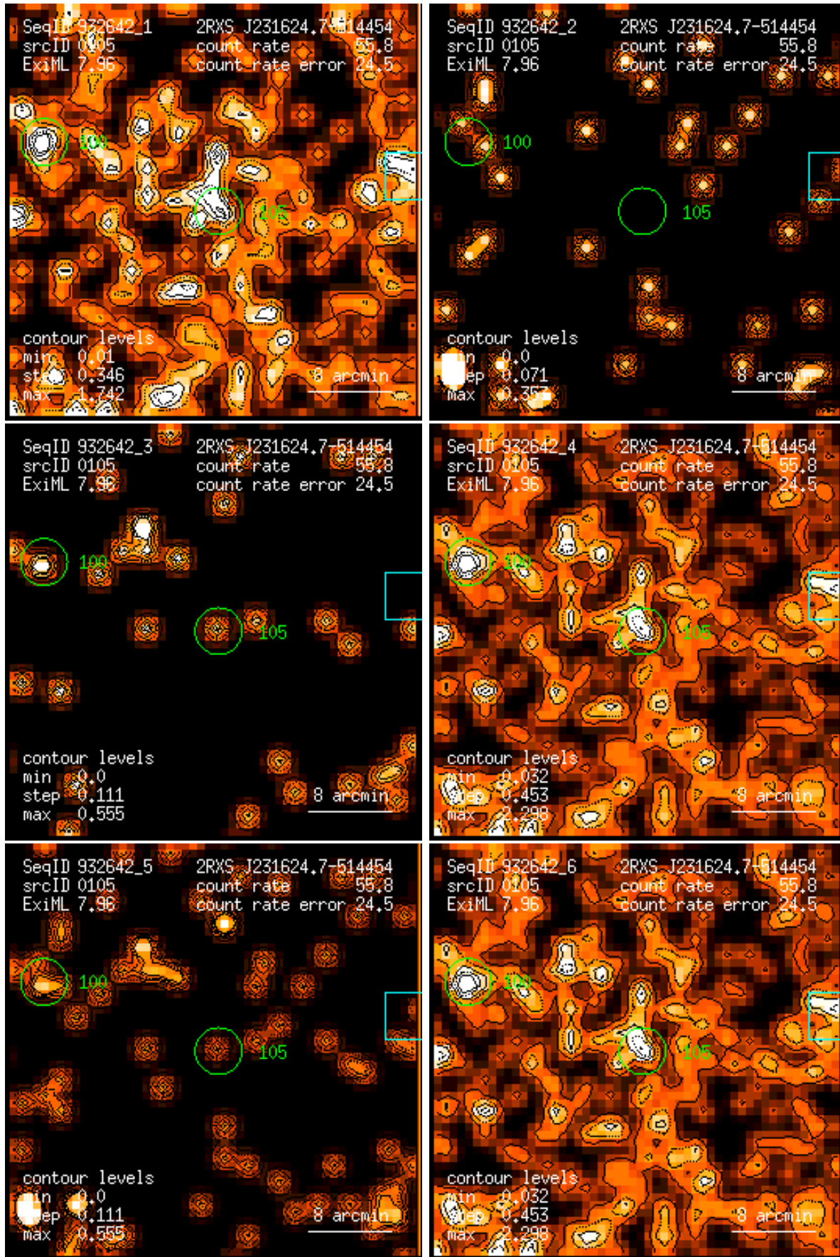
Figure 105: RASS 932642: detection 0105: band rate images, Gaussian filter: (1) PSPC channels 11 – 41, (2) 52 – 90, (3) 91 – 201, (4) 11 – 235, (5) 52 – 201, (6) 11 – 201. Broad band rates in counts/ks. Band rate contour levels in counts/ks/arcmin 2 .
