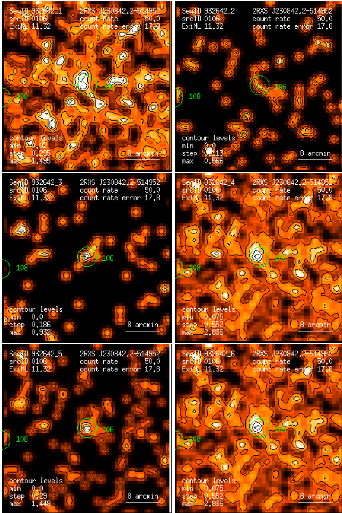
Figure 106: RASS 932642: detection 0106: band rate images, Gaussian filter: (1) PSPC channels 11 – 41, (2) 52 – 90, (3) 91 – 201, (4) 11 – 235, (5) 52 – 201, (6) 11 – 201. Broad band rates in counts/ks. Band rate contour levels in counts/ks/arcmin 2 .
