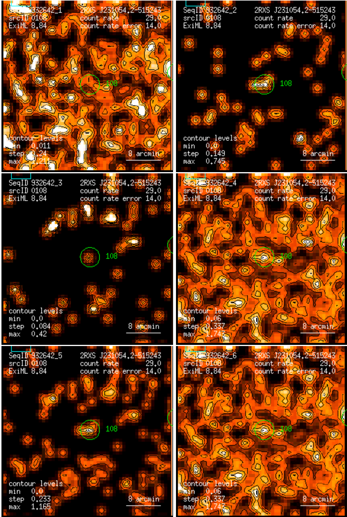
Figure 108: RASS 932642: detection 0108: band rate images, Gaussian filter: (1) PSPC channels 11 – 41, (2) 52 – 90, (3) 91 – 201, (4) 11 – 235, (5) 52 – 201, (6) 11 – 201. Broad band rates in counts/ks. Band rate contour levels in counts/ks/arcmin 2 .
